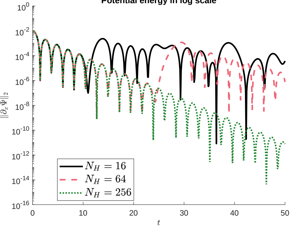
Potential energy in log scale
