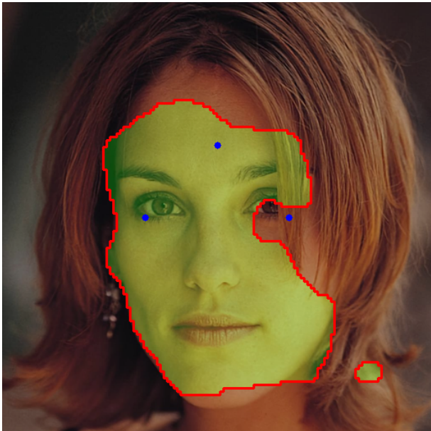
Segmentation Output
