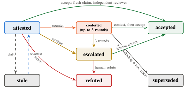
Fig. 2: Claim lifecycle. Solid arrows are ledger appends, dashed arrows are computed from the index. A non-terminal claim becomes stale on binding drift and cannot be accepted until re-attested. Refuted and superseded are terminal.
