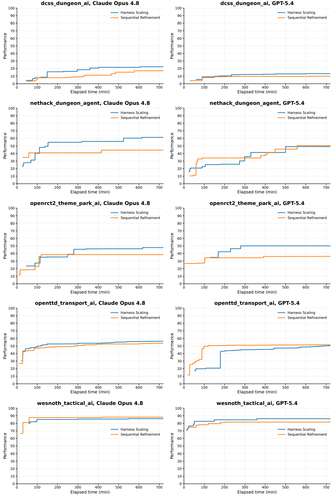
Figure 6: EdgeBench performance over the 12-hour window.
