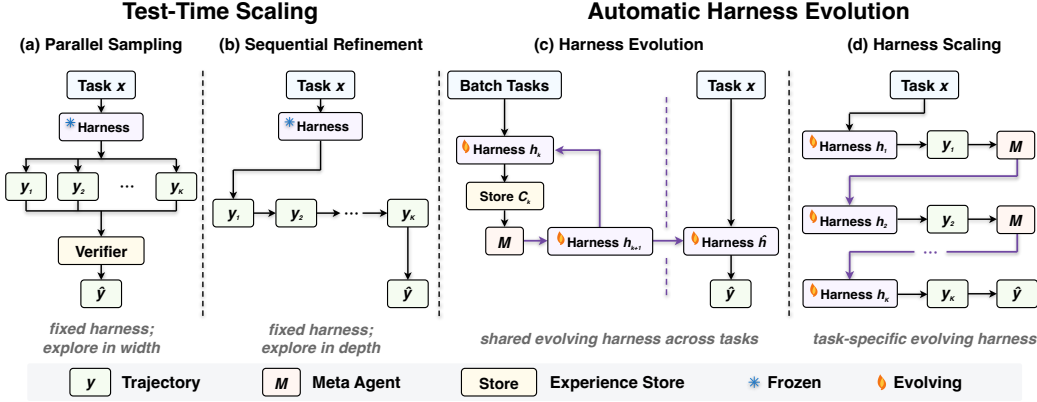
Figure 1: Test-time scaling and automatic harness evolution algorithms. We compare four approaches under a unified budget, emphasizing what feedback the agent receives, how it spends its budget, and whether it modifies the trajectories or the harness.
