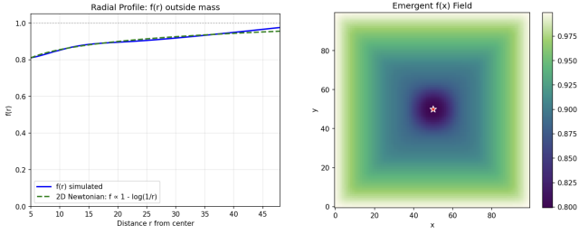
FIG. 4. Steady-state time-sag field for a single localized source on a 2D lattice. (a) Radial profile of f(r) outside the source, compared to the 2D Newtonian prediction f(r) = 1 + \phi(r) with \phi \propto \ln(r/R) , where R is the boundary radius. (b) Emergent f(x) field around the source (star). Darker regions indicate lower completion rate.
