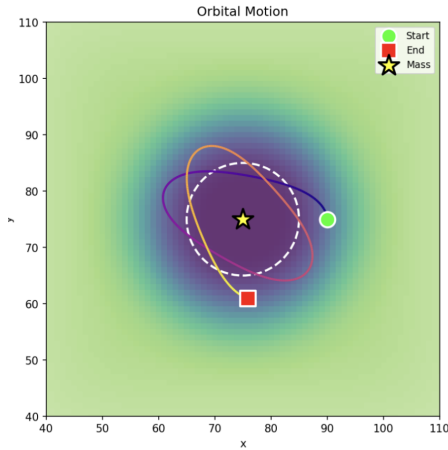
FIG. 5. Orbital motion of a propagating particle around a localized activity source. In a 2D logarithmic potential, orbits precess rather than close.
