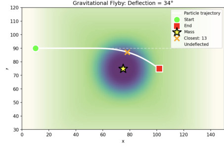
FIG. 6. Gravitational flyby deflection. A particle passing the source at closest approach r_{\min} \approx 13 lattice units is deflected by approximately 34. Dashed line shows the undeflected trajectory.
