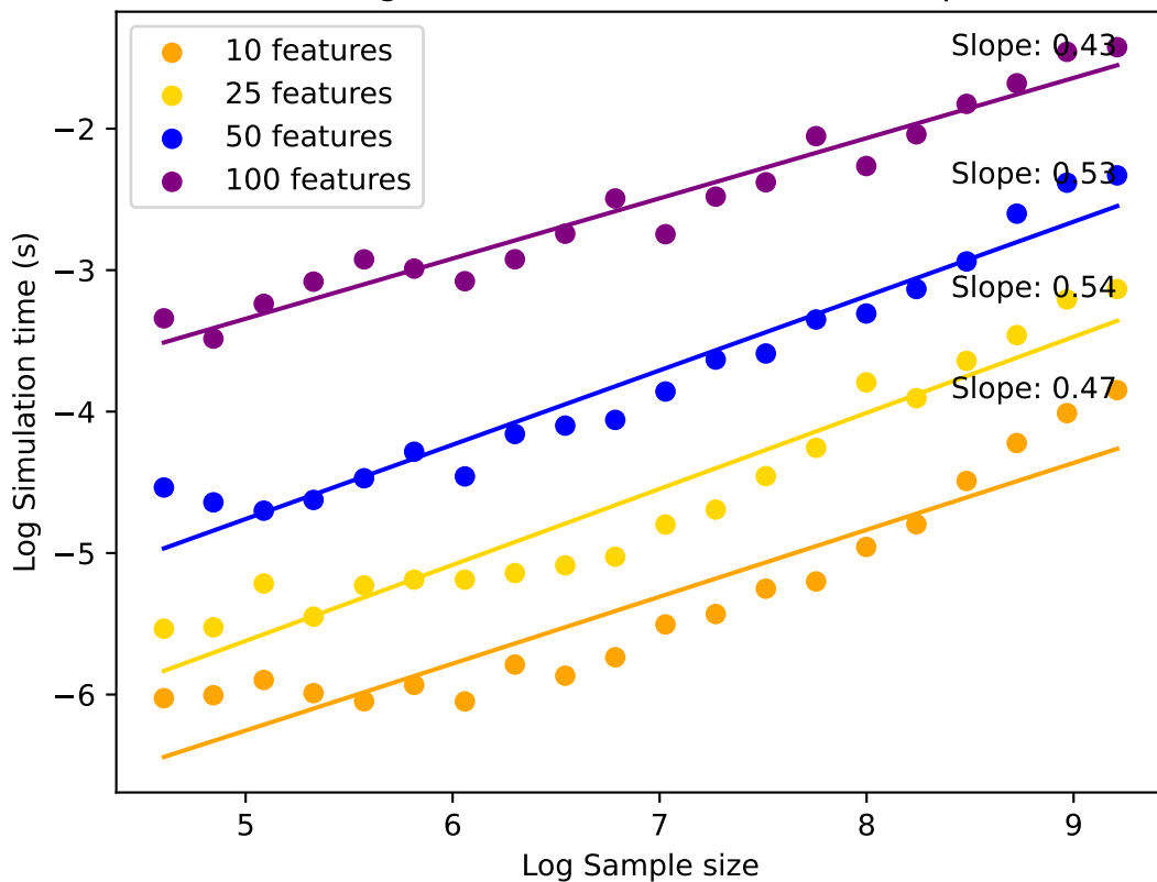
Old average runtime as a function of sample size
