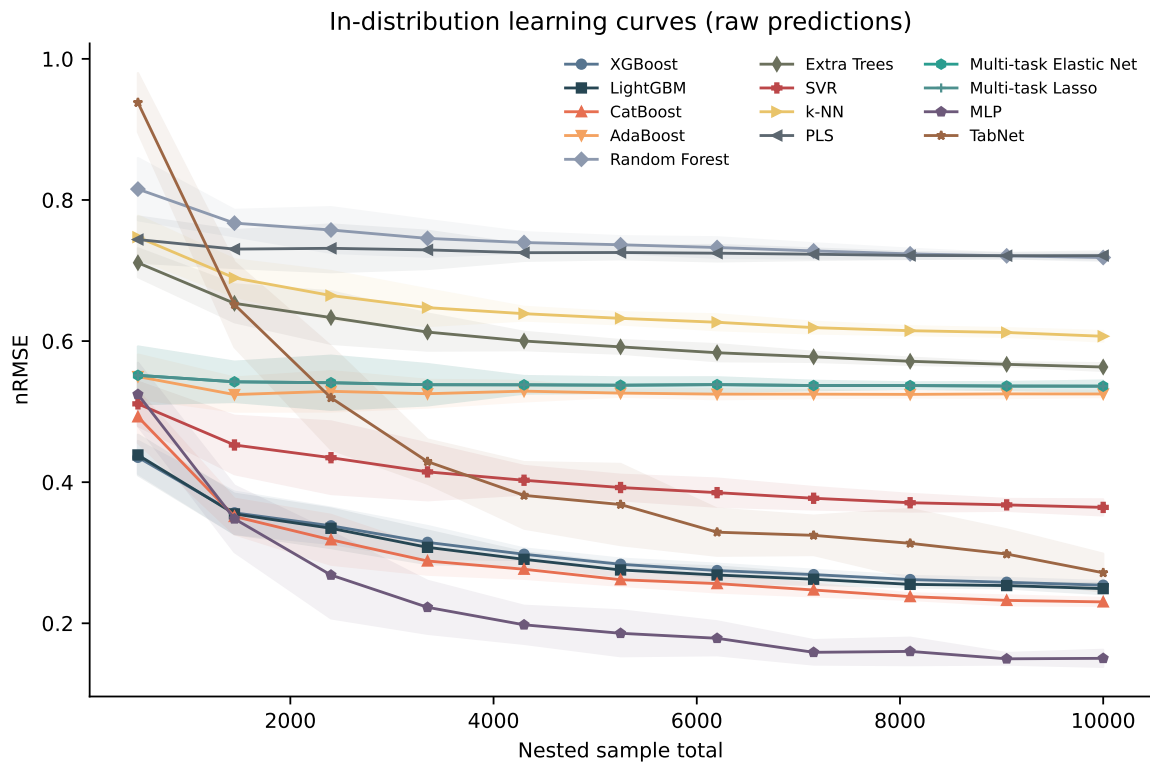
Figure 4.3: Raw component prediction error across the eleven nested design sizes. Lines represent the five-fold mean nRMSE. Shaded regions represent one sample standard deviation across folds.
