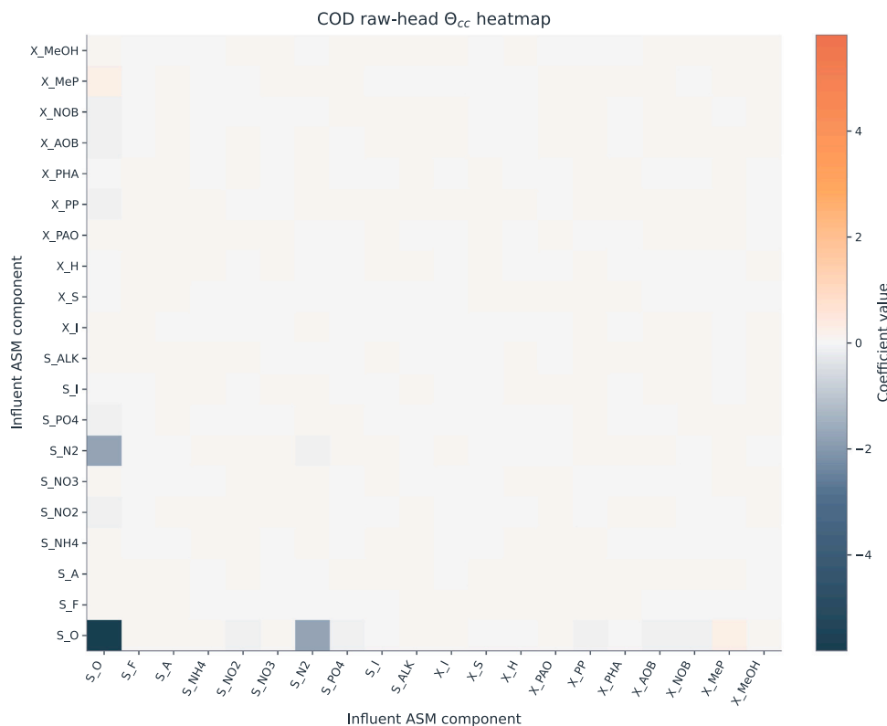
Fig. 4. COD raw-head \Theta_{cc} heatmap from B_{raw,ext} = I_{comp} \hat{R}^{-1} \hat{B} . Rows and columns enumerate influent ASM components. The matrix is symmetric to machine precision; off-diagonal cells are mirrored and each displayed cell is half the coefficient of the corresponding unordered cross term. The full raw-head atlases are reported in Supplementary Figures S1–S4.
