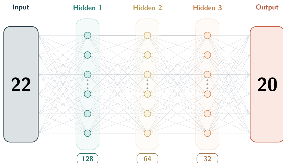
Fig. 1. Architecture of the retained fully connected MLP baseline. The input and output stages are shown as labeled rectangular blocks to distinguish them from the hidden-layer neurons, which are shown as circular vertices. Representative vertices are displayed for the 22-input stage, the three hidden layers of widths 128, 64, and 32, and the 20-component effluent output stage, while the edge pattern indicates dense inter-layer connectivity between successive layers.
