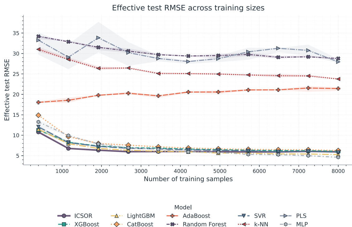
Fig. 2. Repeated dataset-size learning curves from the repeated random train-test evaluations at each retained size. Lines show the mean held-out RMSE across the retained dataset-size sweep, and shaded bands show the interquartile range across the ten repeated runs at each size.
