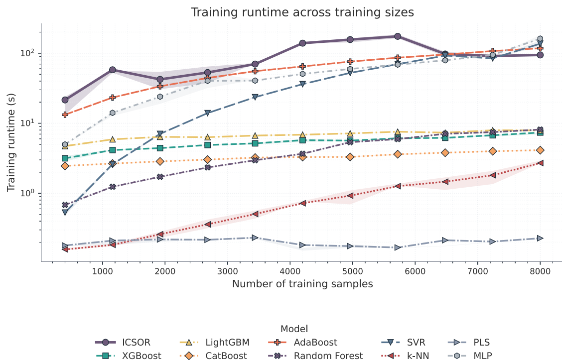
Fig. 3. Repeated dataset-size runtime curves for the retained models. Lines show the mean training time across repeated runs and shaded bands show the interquartile range across the ten repeated runs at each size; the y-axis is logarithmic to keep the full cost spread readable.
