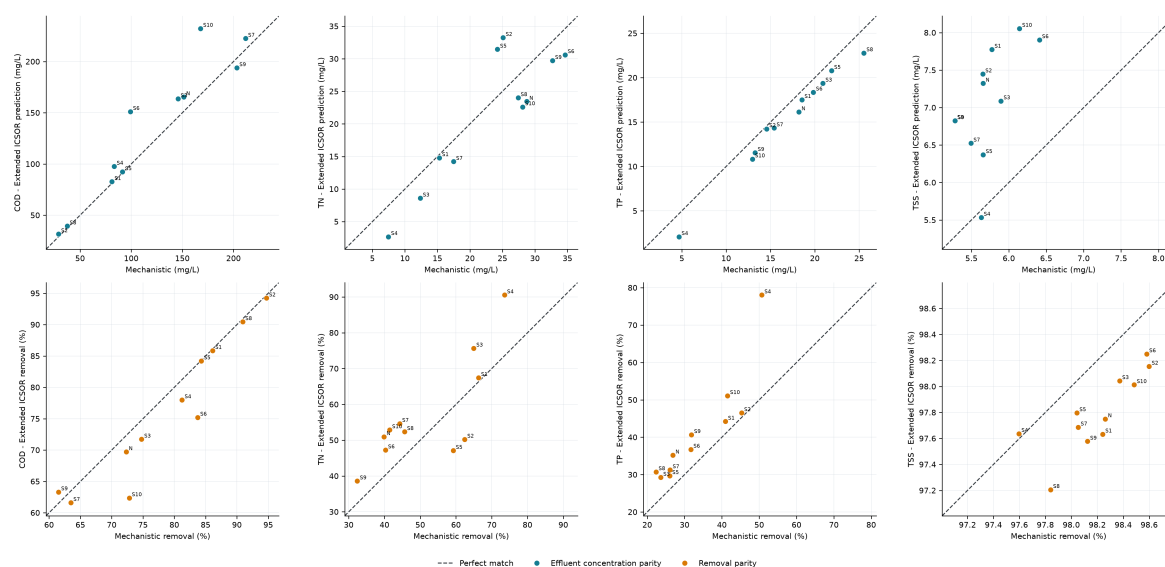
Figure 6.8: Extended ICSOR predictions at selected controls compared with independent original-model evaluation. The upper row shows effluent concentration parity in \text{mg L}^{-1} . The lower row shows removal parity in percent. Columns correspond to COD, TN, TP, and TSS. Teal identifies concentrations and orange identifies removals. Labels identify N and S1–S10. Dashed lines indicate exact agreement.
