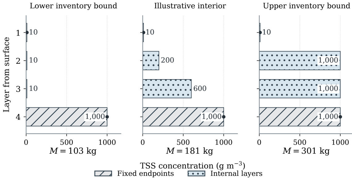
Figure 6.2: Hypothetical four-layer profiles with identical overflow and underflow concentrations. Each layer has volume 100 \text{ m}^3 . The lower-bound, illustrative interior, and upper-bound profiles store 103, 181, and 301 kg of solids. Hatching identifies the fixed endpoints, while dotted fills identify internal layers. The diagram represents the adopted endpoint envelope.
