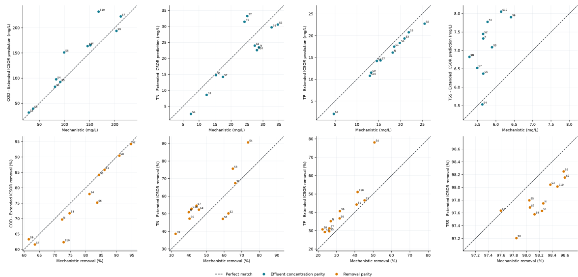
Figure 6.8: Extended ICSOR predictions at selected controls compared with independent original-model evaluation. The upper row shows effluent concentration parity in mg L -1 . The lower row shows removal parity in percent. Columns correspond to COD, TN, TP, and TSS. Teal identifies concentrations and orange identifies removals. Labels identify N and S1–S10. Dashed lines indicate exact agreement.
