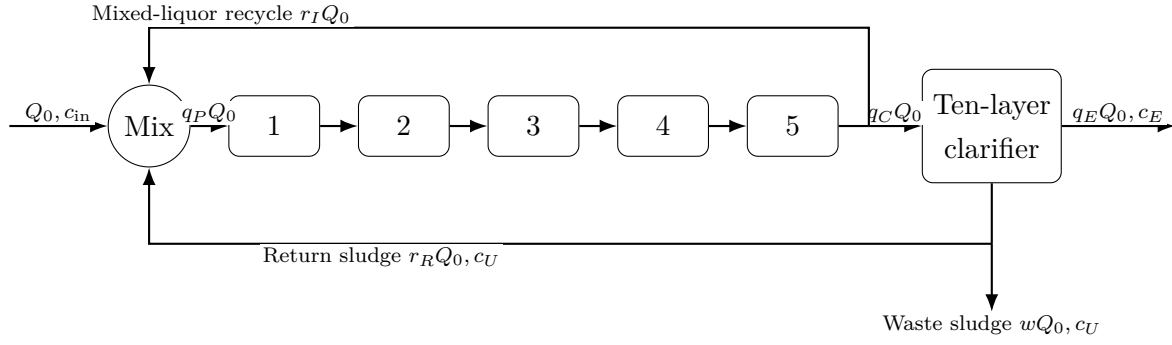
Figure 6.1: Connected plant configuration used for the operating study. Reactors 1 and 2 are unaerated. Reactors 3–5 have independent aeration controls.
