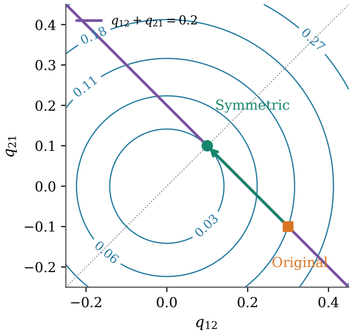
(a) Equal predictions, different norms
