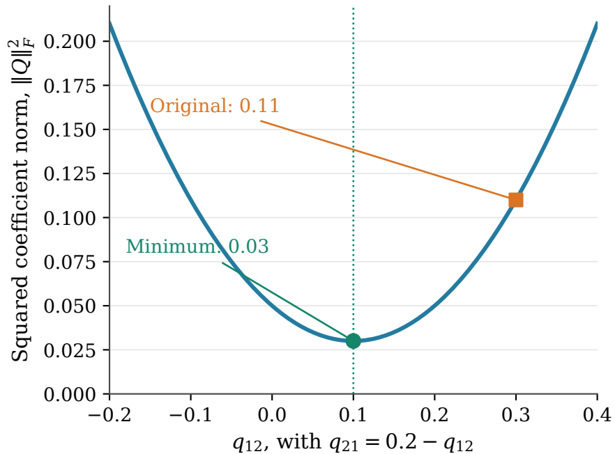
(b) Ridge selects the symmetric point
