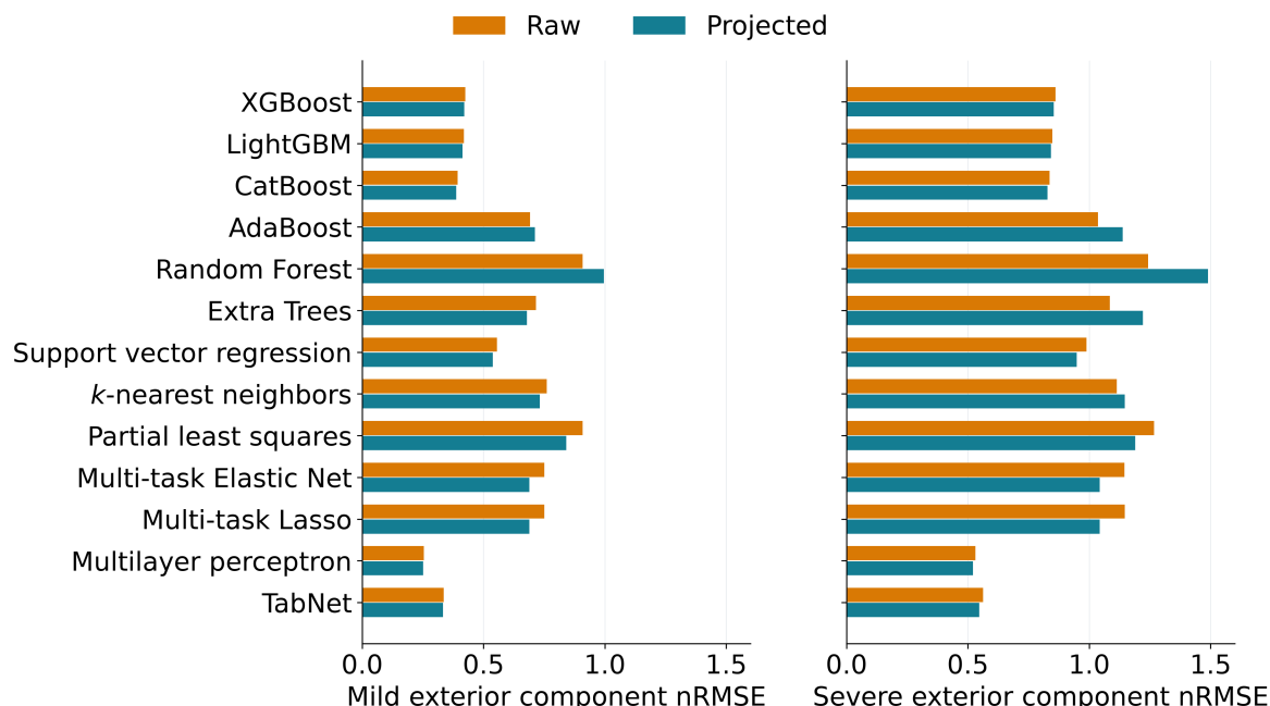
Figure 4.11: Raw and projected component nRMSE for mild and severe exterior inputs. Each severity includes 600 independently simulated reference states. Both panels use full-domain training scales and a common error-axis range.
