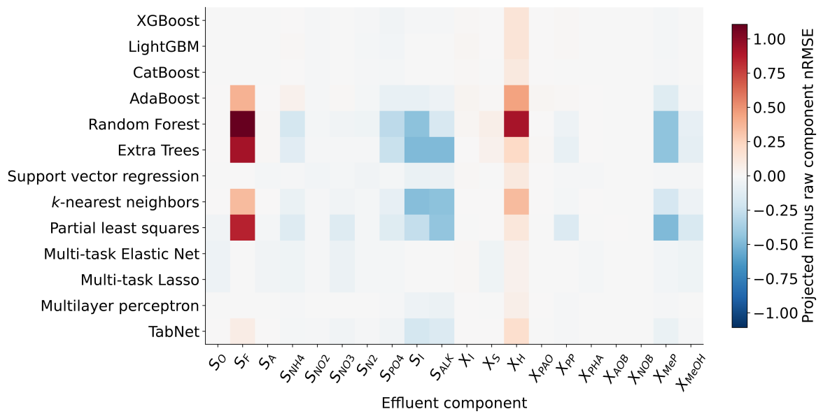
Figure 4.9: Projected minus raw component nRMSE at N = 10,000 . Each cell is the difference between five-fold mean scores for one predictor and one component. Negative values indicate improvement. The same color limits apply to all cells.
