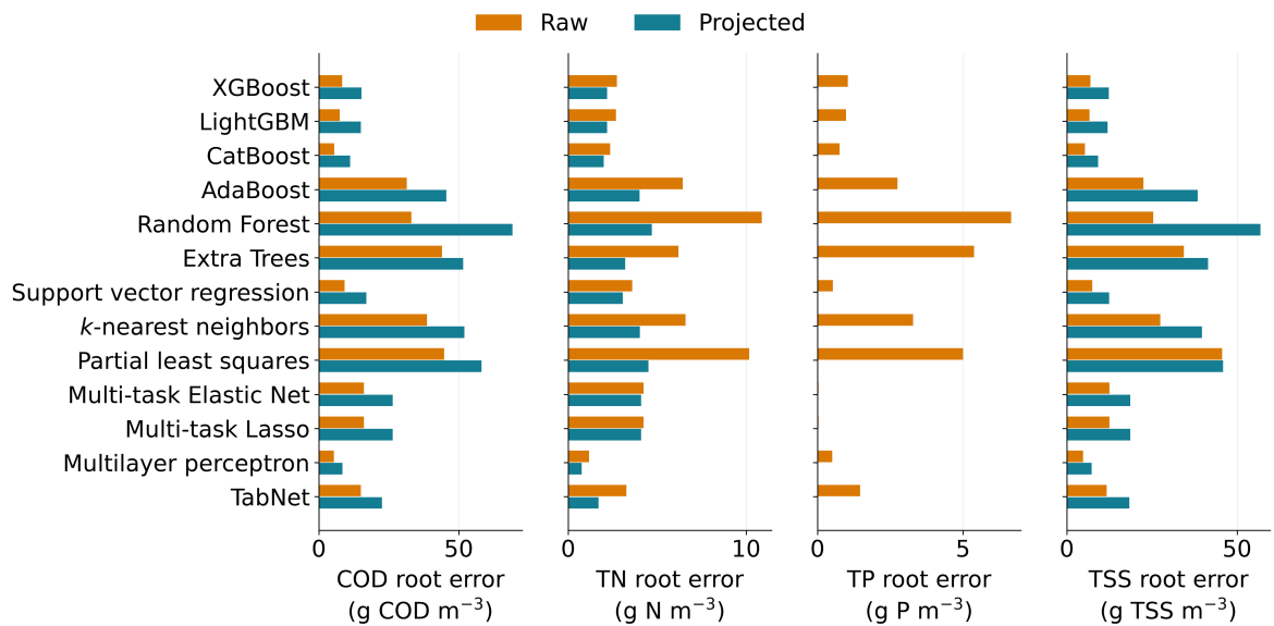
Figure 4.10: Raw and projected root mean squared errors for COD, TN, TP, and TSS at N = 10,000 . Bars show means of five fold-specific root errors. Each panel uses the physical unit of its own reported quantity. These errors are distinct from the standardized component nRMSE.
