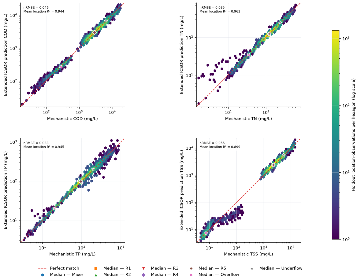
Figure 6.11: Projected composite parity across eight locations and 1845 holdout states. Both concentration axes are logarithmic. Hexagon color gives the number of location-observations, and labelled markers identify each location's median. The one-to-one line indicates exact agreement. Metric annotations retain location-specific normalization and average location-level R^2 .
