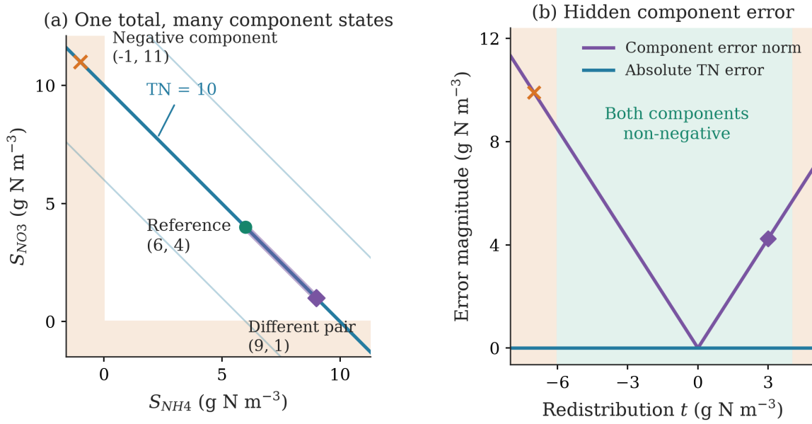
Figure 3.3: Hypothetical geometry of hidden component error under the fixed reporting map. (a) The reference, a pair with different nitrogen components, and a pair with a negative component all give TN of 10 g N m -3 . Pale parallel lines show other TN level sets. (b) Along (6 + t, 4 - t)^T , reported TN error remains zero while component error grows. Teal shading marks the interval where both concentrations are non-negative. Orange shading marks a negative component. All unshown components are zero, and no state is asserted to satisfy the reactor kinetics.
