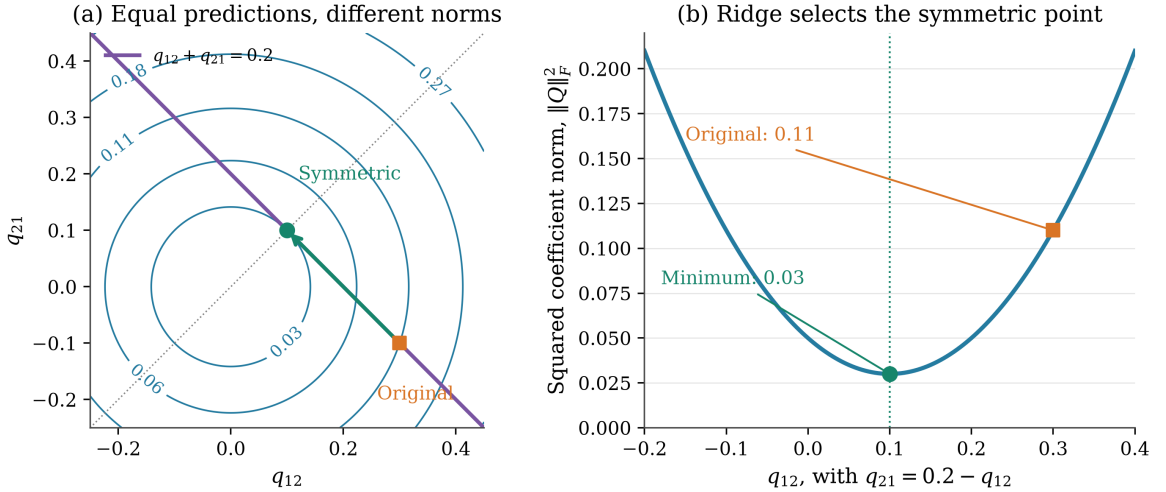
Figure 5.2: Hypothetical coefficient-space geometry of the quadratic matrices in Equation (5.15). The diagonal entries remain q_{11} = 0.1 and q_{22} = 0 . (a) The purple line contains all coefficient pairs with the same unordered interaction coefficient 0.2. Blue contours show \|Q\|_F^2 = 0.01 + q_{12}^2 + q_{21}^2 . The original orange point and symmetric teal point have squared norms 0.11 and 0.03. (b) Restricting this norm to the equal-response line gives a quadratic minimum at q_{12} = q_{21} = 0.1 . This construction illustrates the norm decomposition in Equation (5.17).
