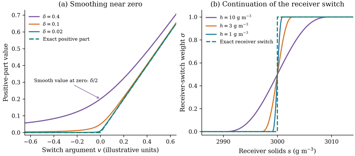
Figure 6.7: Analytical illustration of smoothing near process switches. (a) The positive-part approximation in Equation (6.171) for illustrative widths \delta = 0.4, 0.1, 0.02 , which are chosen for visibility and are not the numerical continuation settings. (b) The quintic receiver switch in Equation (6.174) at the illustrative threshold X_t = 3000 \text{ g m}^{-3} , using the continuation half-widths h = 10, 3, 1 \text{ g m}^{-3} . Dashed curves show the original branch mappings. The vertical receiver-switch line represents its jump rather than an intermediate physical branch value.
