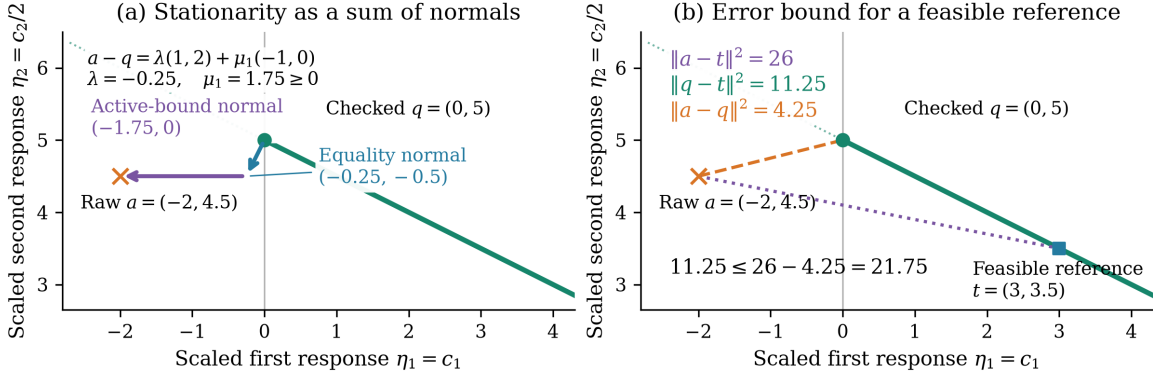
Figure 6.5: Hypothetical geometric interpretation of the projection certificate and its error bound, with coordinate scales (1, 2) . The solid teal line shows the visible portion of the non-negative segment of \eta_1 + 2\eta_2 = 10 . The dotted extension satisfies only the equality. (a) Equality and active-bound normal contributions, drawn head to tail, sum to the displacement from the checked state to the raw prediction. (b) The triangle compares squared distances to the feasible reference (3, 7) in physical coordinates. All displayed distances use scaled coordinates. The error guarantee applies to this complete feasible set and this metric.
