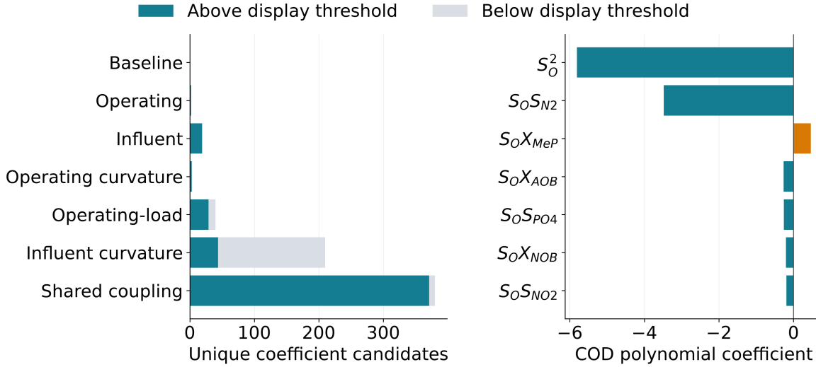
Figure 5.14: Coefficient structure of one fitted ICSOR model. The left panel separates entries above and below the display thresholds for the COD polynomial blocks and shared coupling. The right panel shows selected COD influent-curvature coefficients with mirrored interaction entries combined. Coefficient units depend on the corresponding input terms. The displayed values describe the raw composite mapping.
