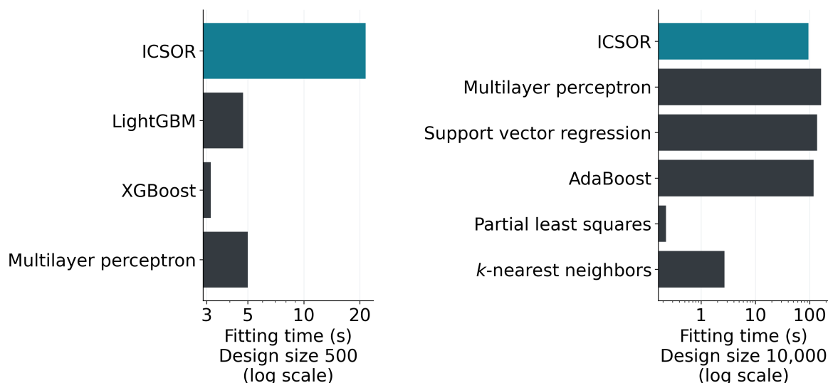
Figure 5.13: Mean fitting times for the specified predictors at design sizes 500 and 10,000. Teal identifies ICSOR. Each panel uses a logarithmic seconds axis. The values concern repeated model fits and exclude deployment calculations.
