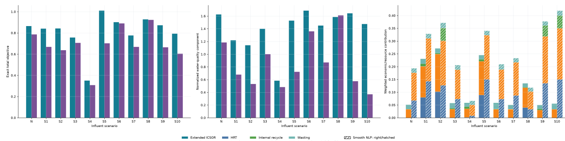
Figure 6.15: Common-reference total objective, normalized quality cost, and weighted resource contributions. Both routes are evaluated with the original mechanistic model and common quality scales. Resource stacks show HRT, aeration, internal recycle, return sludge, and wasting. Solid bars identify Extended ICSOR, and hatched bars identify Smooth NLP. The quality panel shows j_Q , whose contribution to the total objective is 0.50j_Q .
