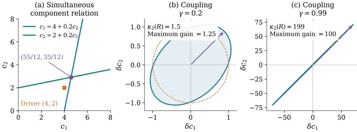
Figure 5.3: Hypothetical geometric interpretation of simultaneous component coupling and numerical conditioning. (a) The lines in Equation (5.18) intersect at (55/12, 35/12) . The orange square marks the driver (4, 2) . (b,c) For symmetric two-component coupling 0.2 and 0.99, respectively, the blue ellipse is \delta c = R^{-1}\delta r with \|\delta r\|_2 = 1 . The dashed orange unit circle supplies the unamplified reference. Purple arrows show the direction of maximum gain. The two perturbation panels use different axis ranges to show gains of 1.25 and 100, with condition numbers 1.5 and 199. The unit circle consequently appears tiny in panel (c). The nearly singular example illustrates a numerical failure mode and does not satisfy the adopted entry bound in Equation (5.22).
