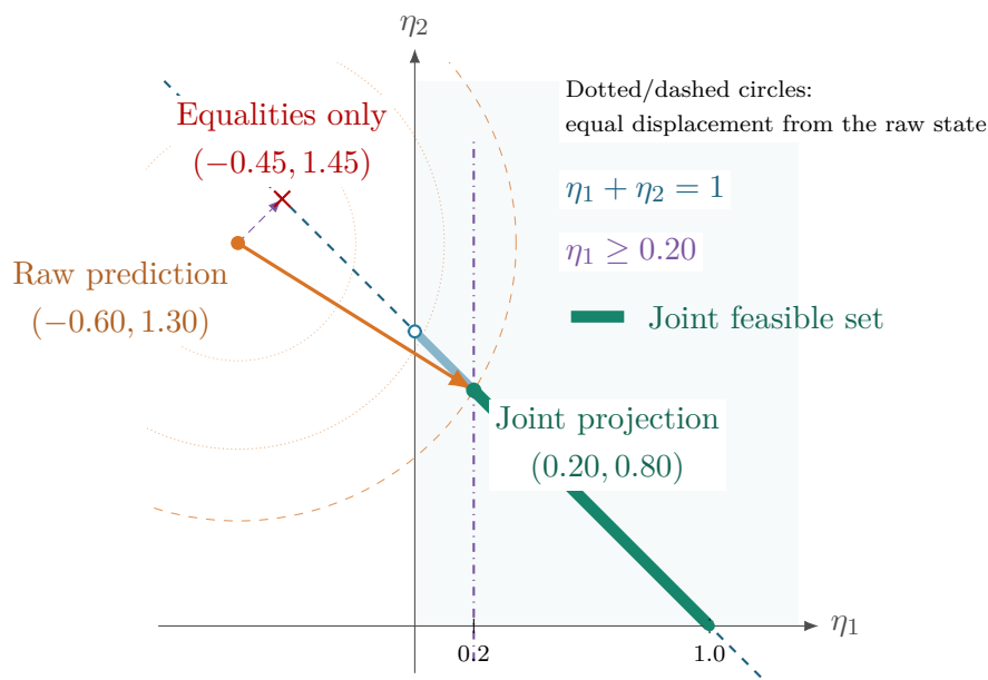
Figure 6.4: Analytical illustration of joint plant-response projection in two scaled coordinates. The equality line, non-negativity and an additional inequality intersect to form the green feasible segment. The orange arrow gives the shortest admissible correction from the raw point, while the red cross shows an equality-only projection that remains negative. Circles denote equal standardized displacement from the raw point. The illustration explains the projection criterion and is not a simulated plant result.
