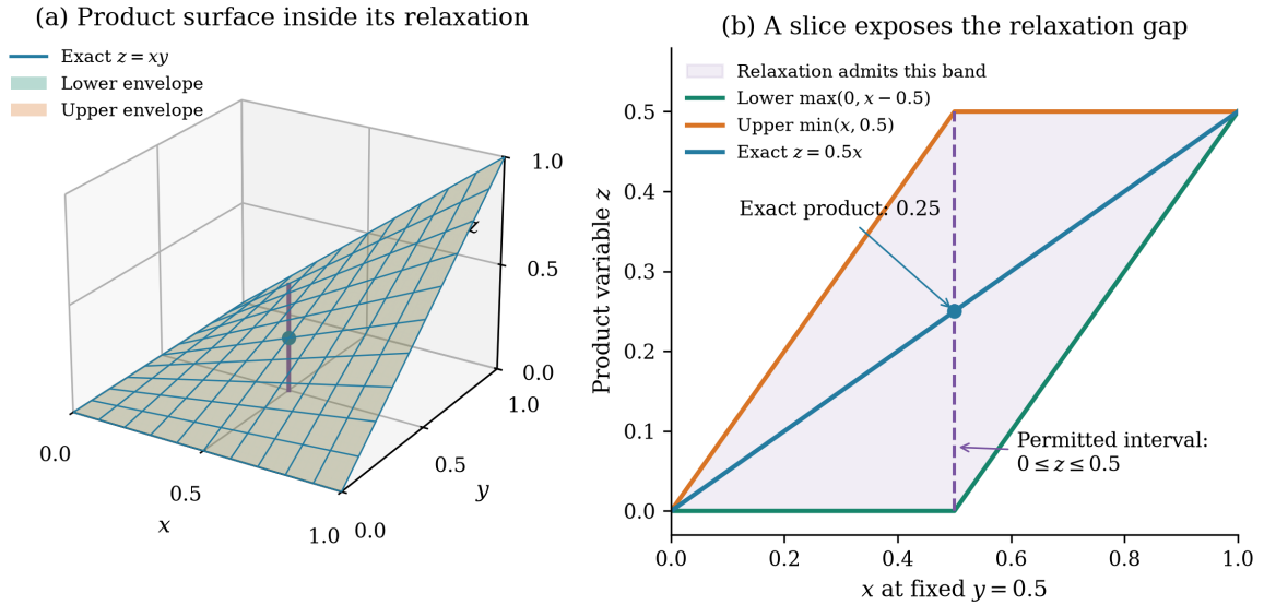
Figure 6.6: Analytical illustration of a McCormick relaxation for the hypothetical unit box 0 \leq x, y \leq 1 . (a) The exact surface z = xy lies between the lower envelope \max(0, x + y - 1) and upper envelope \min(x, y) . (b) A slice at y = 0.5 shows the interval admitted by the relaxation. At x = 0.5 , only z = 0.25 is the exact product, although the relaxed inequalities admit the entire interval [0, 0.5] .
