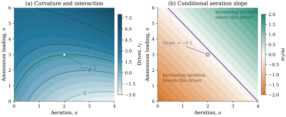
Figure 5.1: Hypothetical geometric interpretation of the second-order driver in Equation (5.13), with coefficients (1, -2, 0.5, 0.25, 0.3) in its stated coefficient order. Inputs and driver values use illustrative units. (a) The contours show equal driver response. The teal curve passes through (a, n) = (2, 3) , where r_f = 1.3 . (b) The conditional aeration slope is -2 + 0.5a + 0.3n . Orange and teal indicate negative and positive slopes, respectively, and the purple line marks zero slope. The figure illustrates a statistical driver before component coupling and physical enforcement.
