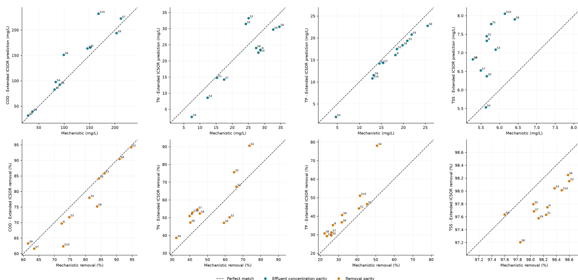
Figure 6.12: Extended ICSOR predictions at selected controls compared with independent original-model evaluation. The upper row shows effluent concentration parity in \text{mg L}^{-1} . The lower row shows removal parity in percent. Columns correspond to COD, TN, TP, and TSS. Teal identifies concentrations and orange identifies removals. Labels identify N and S1–S10. Dashed lines indicate exact agreement.
