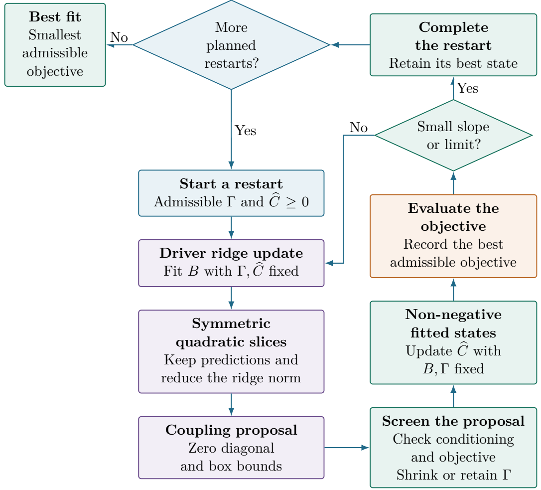
Figure 5.4: Conceptual fitting cycle with explicit symmetry, conditioning, descent, and non-negativity checks. The prescribed restart count can be one.
