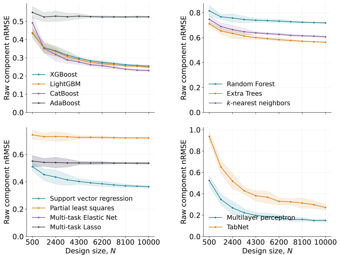
Figure 4.6: Raw component prediction error across the eleven nested design sizes. Separate panels group the predictors by their response representation. Lines show the five-fold mean nRMSE. Shaded regions show one sample standard deviation across folds.
