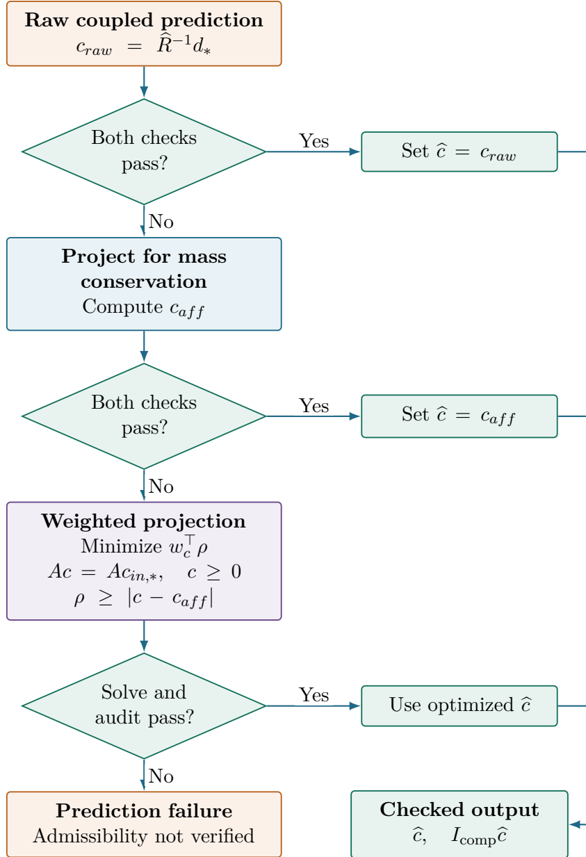
Figure 5.5: Checked deployment of one predicted component state. Accepted branches merge before the common reporting map is applied. A failed final audit produces a reported prediction failure.
