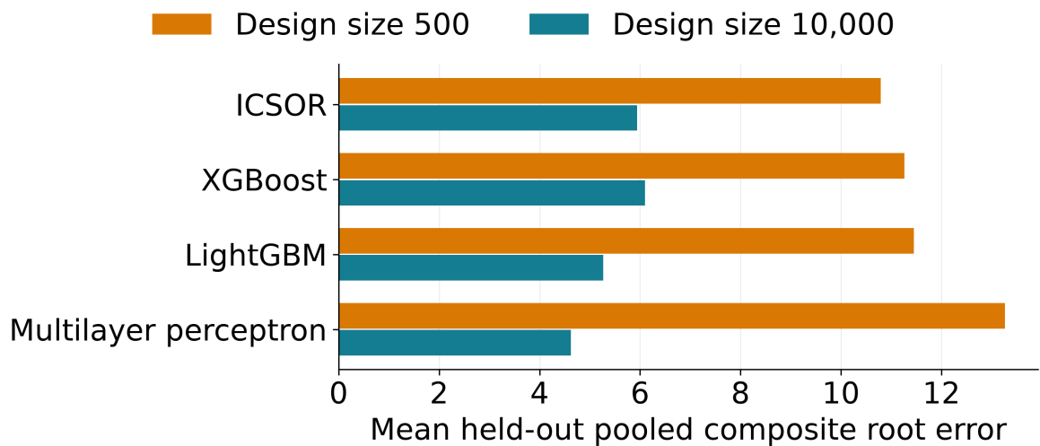
Figure 5.11: Mean held-out pooled composite root error at design sizes 500 and 10,000 for ICSOR, XGBoost, LightGBM, and the multilayer perceptron. Values summarize ten repeated splits. The panels show repeated-split endpoint means at the two specified design sizes.
