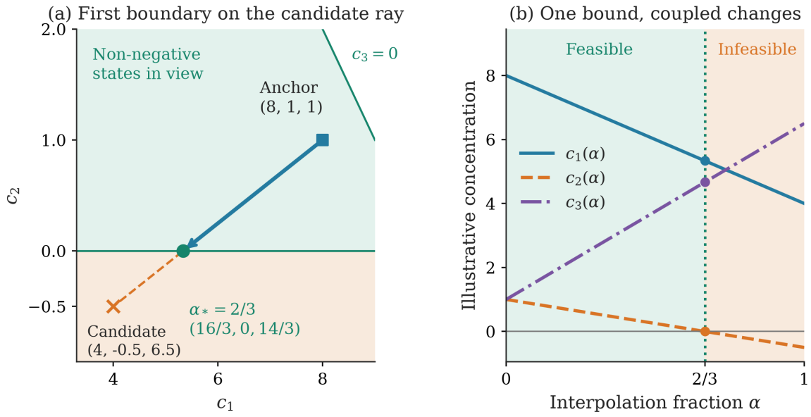
Figure 4.3: Hypothetical largest-feasible-interpolation geometry for the anchor (8, 1, 1)^\top and mass-conserving candidate (4, -0.5, 6.5)^\top . (a) The blue ray stops at the first concentration boundary, returning (16/3, 0, 14/3)^\top . The dashed continuation reaches the negative candidate. Shading shows a local portion of the non-negative set in the inventory plane. (b) Every coordinate uses the same fraction, and the inventory remains 10 throughout. The common illustrative concentration basis permits this simple sum. The numerical safety margin is omitted for visibility.
