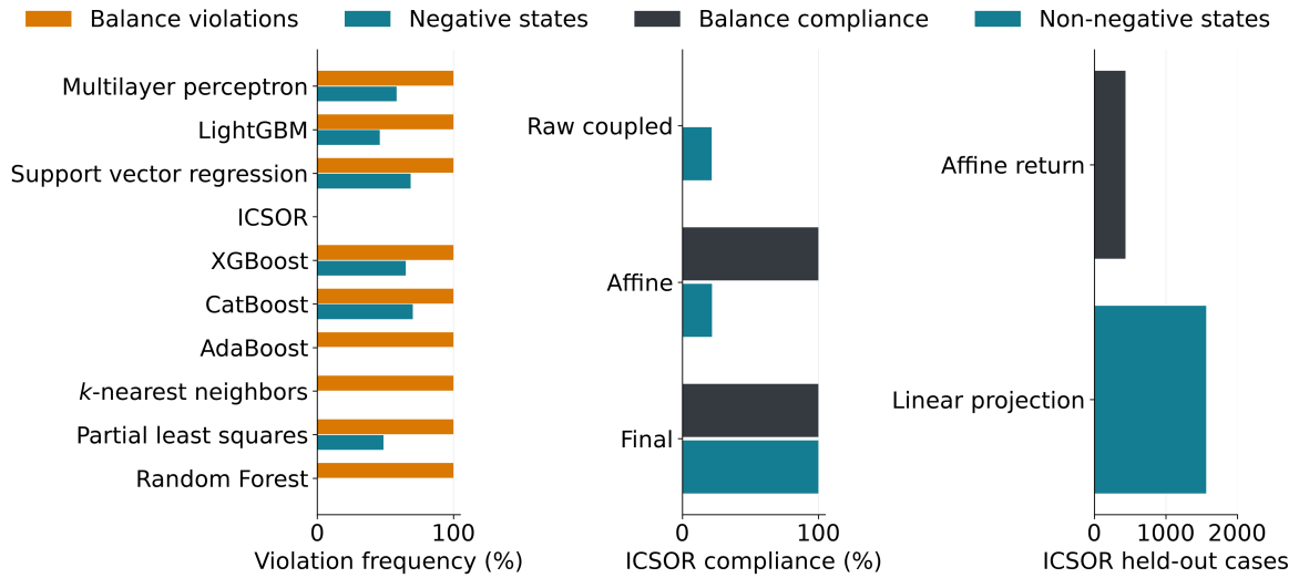
Figure 5.12: Physical diagnostics and ICSOR deployment on 2000 held-out cases. The left panel compares final ICSOR states with raw comparator states. The middle panel separates raw coupled, affine, and final ICSOR compliance. The right panel gives the numbers returned after affine projection and after constrained linear projection. Balance checks use the adopted numerical operator A_{num} .
