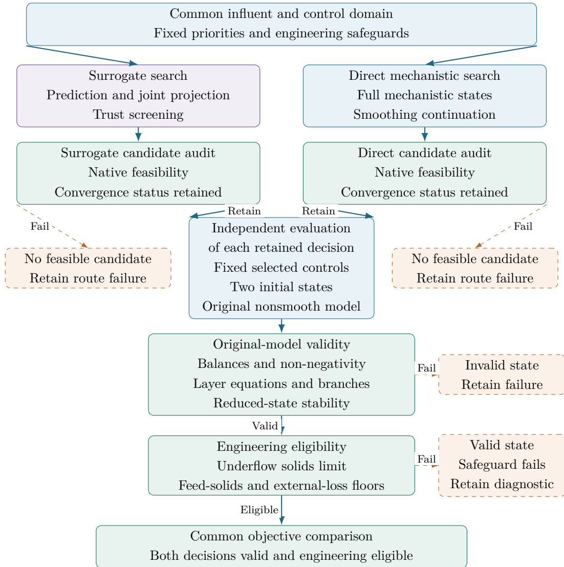
Figure 6.8: Conceptual paired-search and verification workflow. Each retained control vector receives its own independent original-model evaluation. The surrogate and smooth-direct native responses do not supply the reference treatment outcome. Original-model validity and engineering eligibility are distinct checks. Only eligible pairs enter the common-objective comparison, while failed or qualified cases remain in the accounting.
