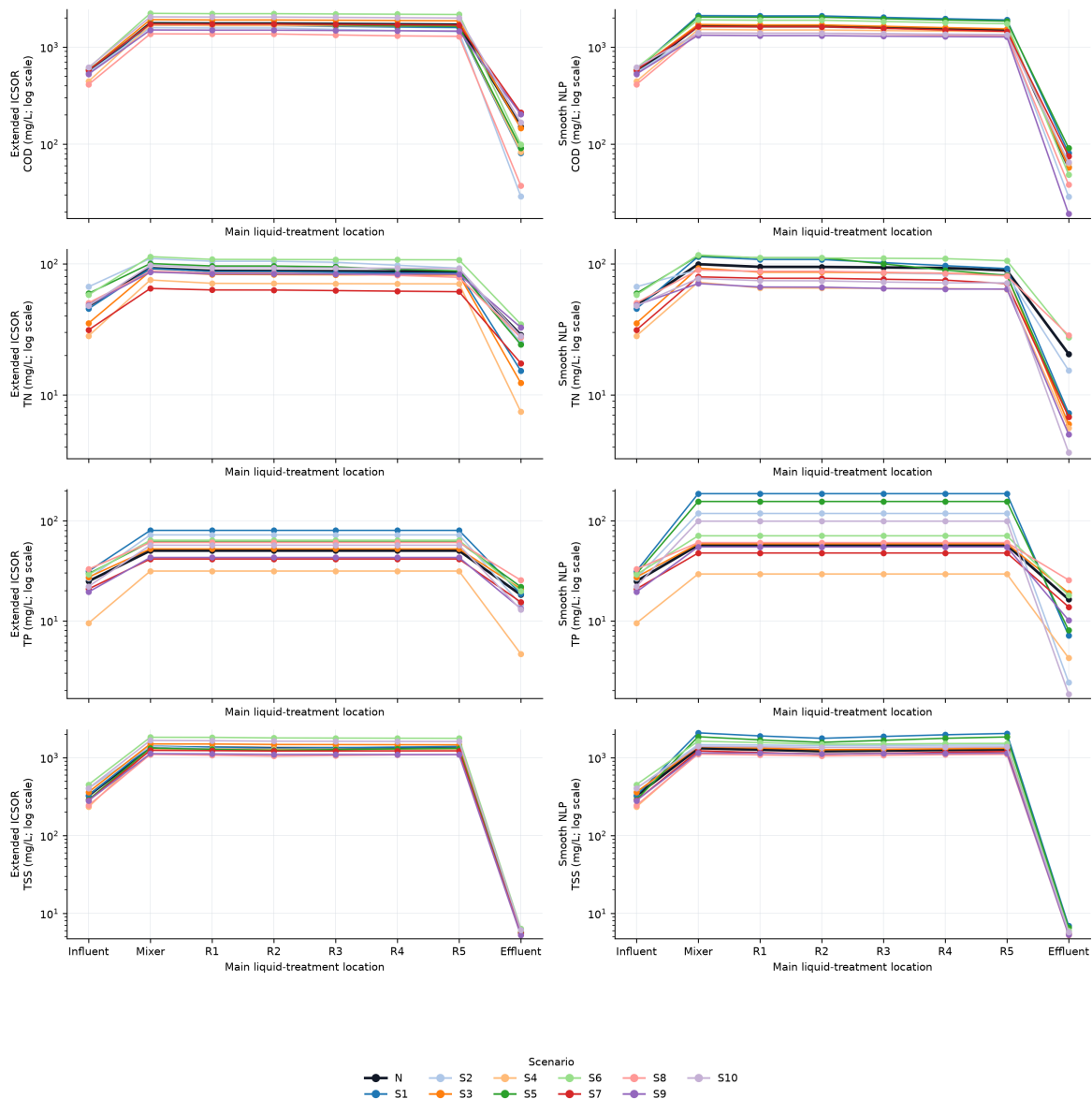
Figure 6.14: Mechanistic concentration profiles at controls selected by Extended IC-SOR and Smooth NLP. Rows show COD, TN, TP, and TSS from fresh influent through the mixer and reactors 1–5 to clarifier effluent. Each composite has identical logarithmic concentration limits for both routes. Colors identify N and S1–S10. Underflow is not placed in the main liquid-treatment path.
