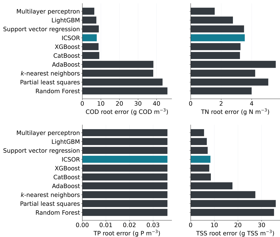
Figure 5.9: Fixed-split root mean squared error for COD, TN, TP, and TSS. Teal identifies ICSOR and gray identifies the comparators. Each panel has its own constituent unit and horizontal scale. All methods have the same reported TP error under the specified alignment and reporting procedure.
