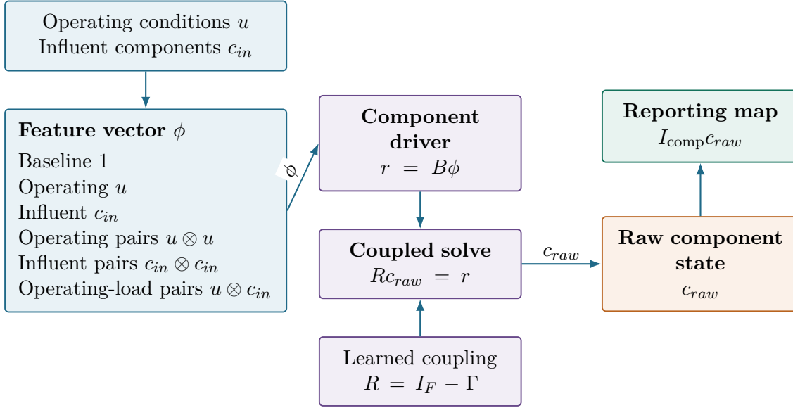
Figure 5.6: Named feature blocks and the transformation from driver to raw component and reported-composite predictions. Composing the three operations gives the raw reported coefficient map I_{\text{comp}}R^{-1}B .
