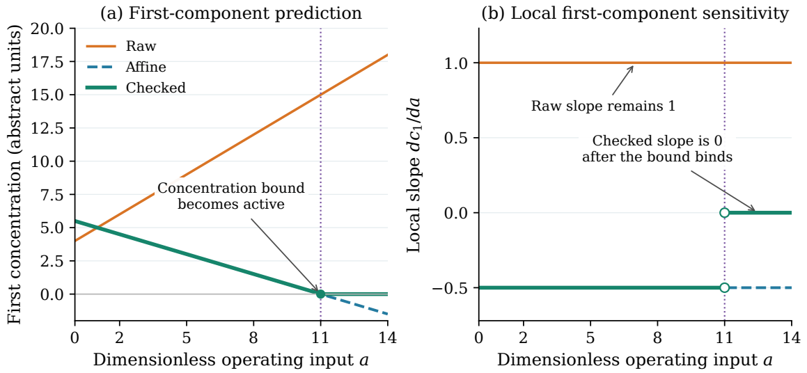
Figure 5.7: Hypothetical first-component response and sensitivity before and after mass conservation and non-negativity enforcement. Open circles mark the two one-sided checked slopes at the active-boundary transition.
