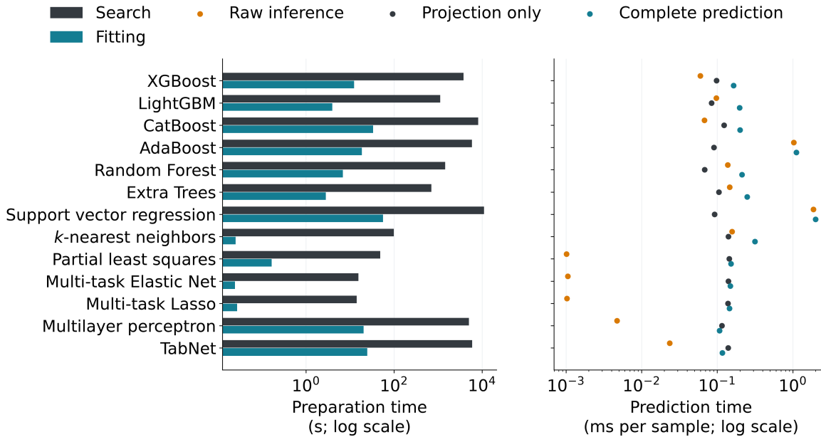
Figure 4.12: Model preparation and repeated prediction costs at N = 10,000 . The left panel separates search and fitting in seconds. The right panel separates raw inference, projection alone, and complete prediction in milliseconds per sample under the fixed batch protocol. Both panels show five-fold means on logarithmic axes. Complete prediction was timed separately.
