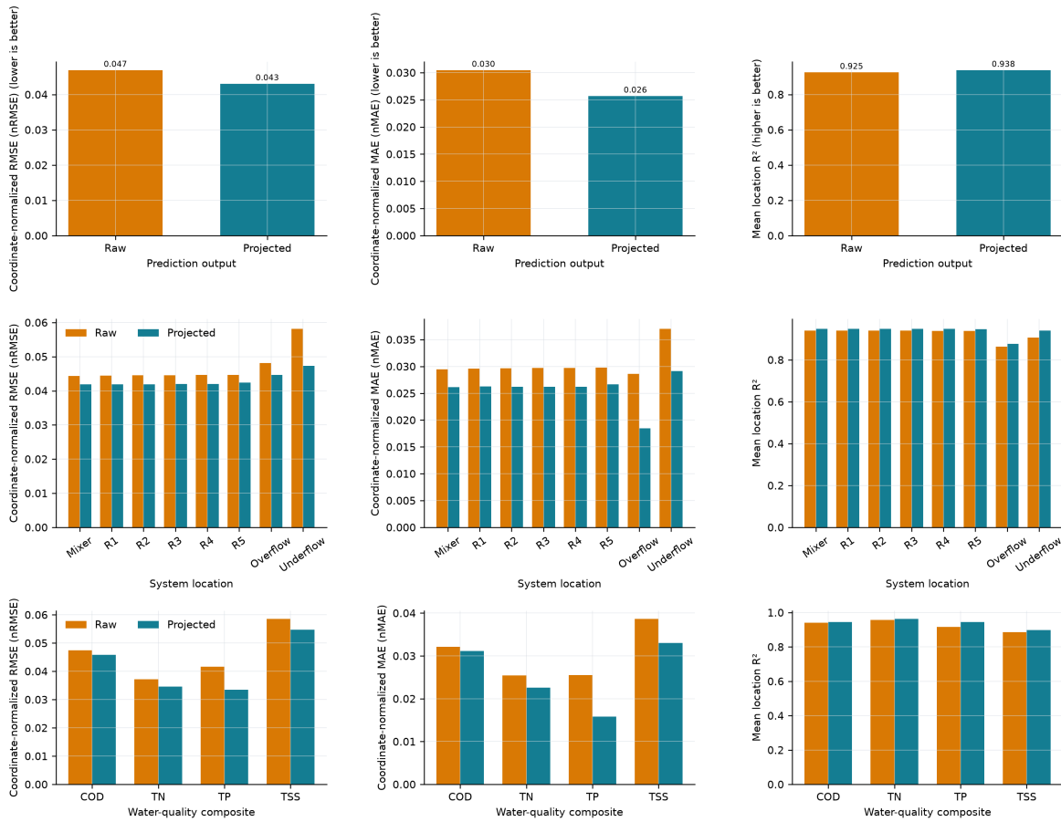
Figure 6.9: Raw and projected composite accuracy on 1845 holdout plant states. Rows show aggregate, location, and composite summaries. Columns show nRMSE, nMAE, and mean location-level R^2 . Errors are normalized by the mechanistic holdout range of each location and composite. The R^2 summaries average coordinate-specific scores rather than pooling locations into one score.
