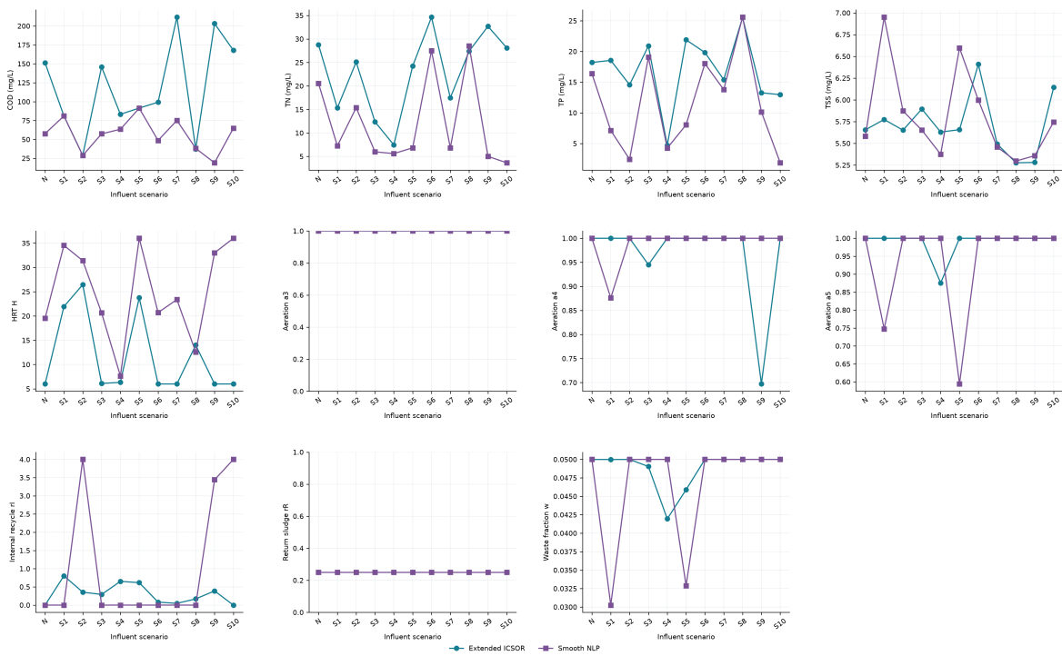
Figure 6.13: Mechanistic effluent outcomes and selected controls for both optimization routes. The top row shows COD, TN, TP, and TSS in \text{mg L}^{-1} . The remaining panels show HRT, aeration in reactors 3–5, internal recycle, return sludge, and wasting. The unused panel is omitted. N and S1–S10 appear in every comparison. The constant aeration and return-sludge panels use plain zero-to-one axes.
