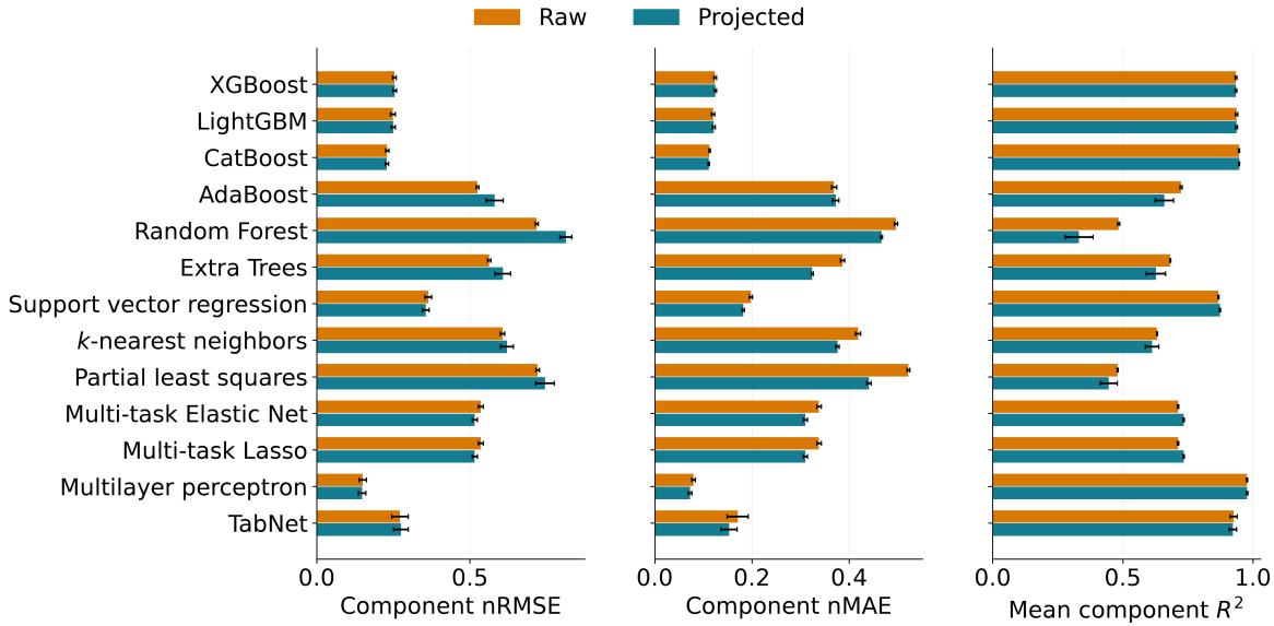
Figure 4.5: Raw and projected component accuracy at N = 10,000 . Panels show nRMSE, nMAE, and the mean component R^2 . Error bars show one sample standard deviation across five outer folds.
