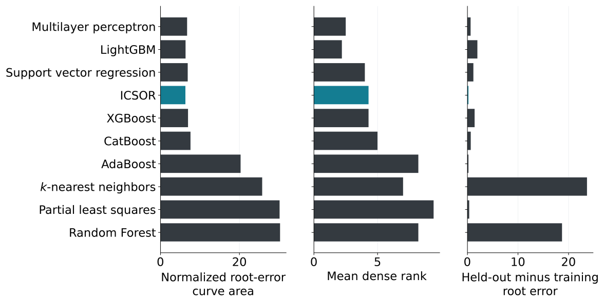
Figure 5.10: Normalized root-error curve area, mean dense rank, and held-out minus training root-error gap. Curve areas and ranks summarize eleven design sizes with ten repeated splits per size. The gap refers to the largest design size. Teal identifies ICSOR. The gap is reported alongside the held-out error.
