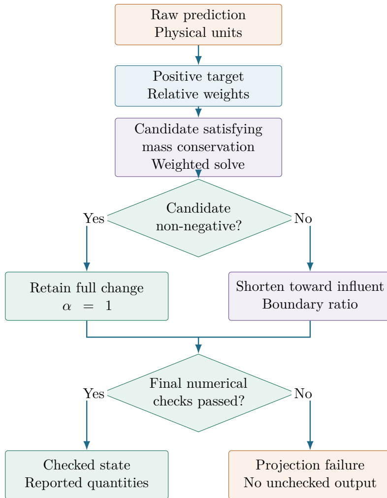
Figure 4.4: Post prediction mass conservation and non-negativity procedure. Positive-target construction, projection for mass conservation, and final-state acceptance have separate roles. The diagram shows the sequence used for each prediction.
