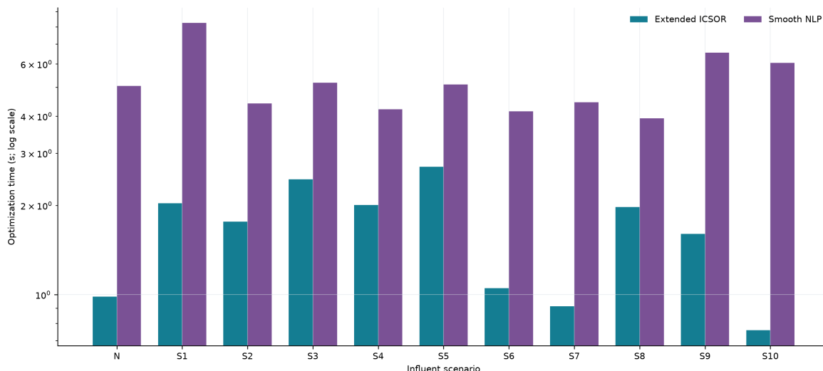
Figure 6.16: Recorded optimization time for N and S1–S10 on a logarithmic seconds axis. The interval includes the initial surrogate search with projection and fallback or the initial direct smoothing sequence. It excludes generation, fitting, certification, conditional recovery, and independent mechanistic evaluation. Initial failed attempts remain in the timing account. Scenario mean times use S1–S10 only.
