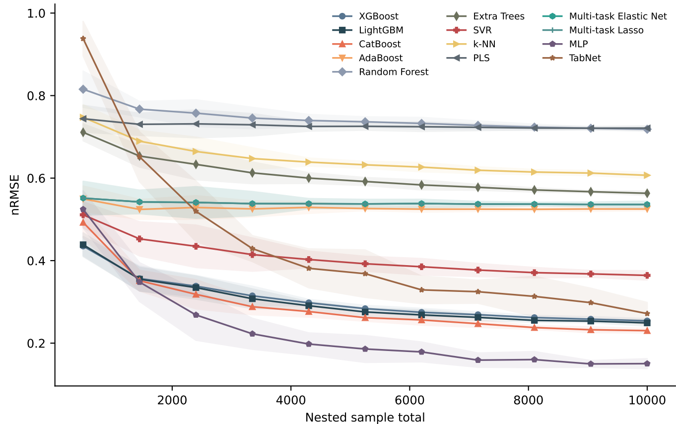
In-distribution learning curves (raw predictions)
