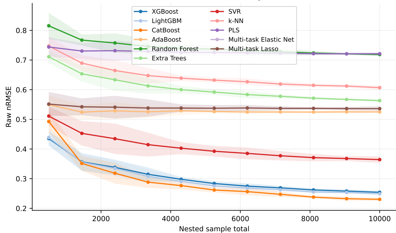
Five-fold in-distribution learning curves
