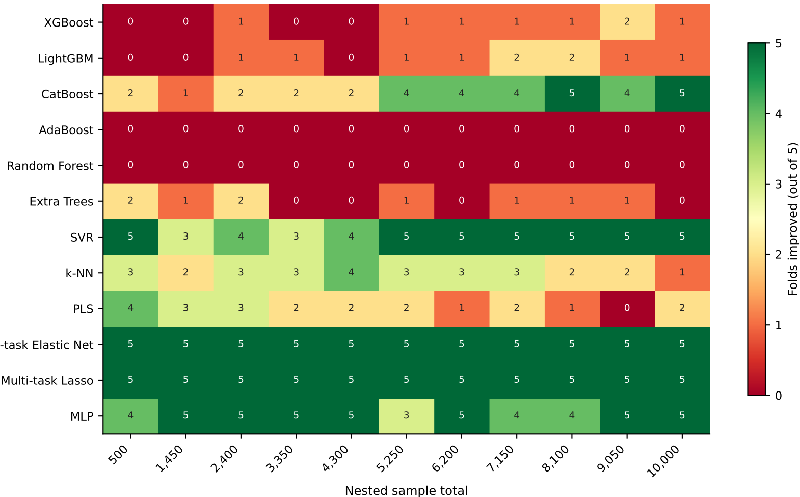
How consistently does projection improve nRMSE across the five folds?
