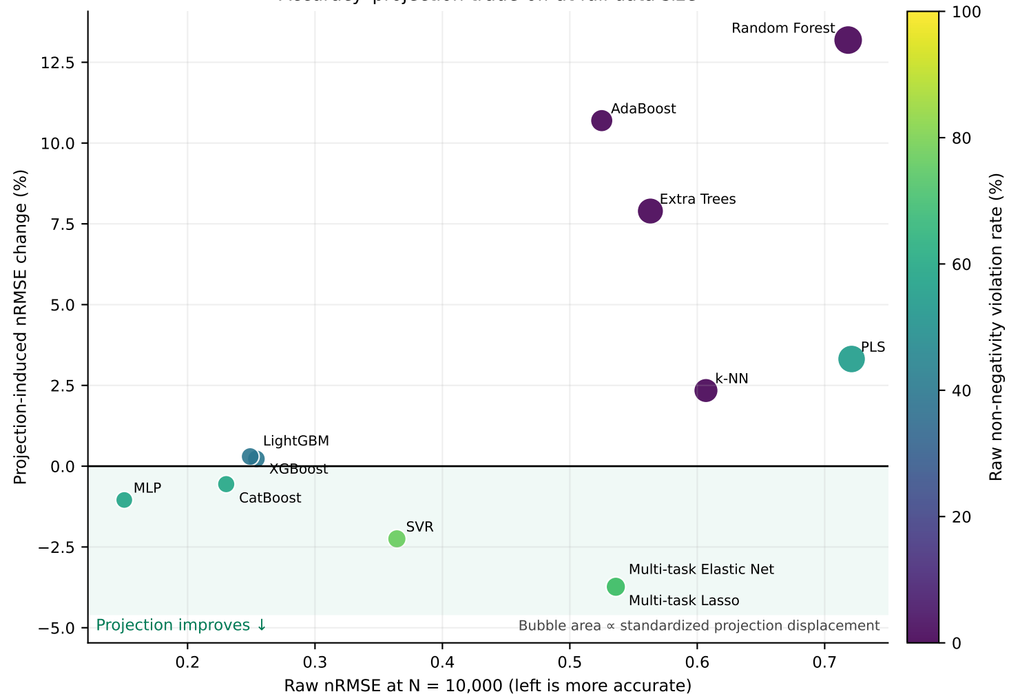
Accuracy-projection trade-off at full data size
