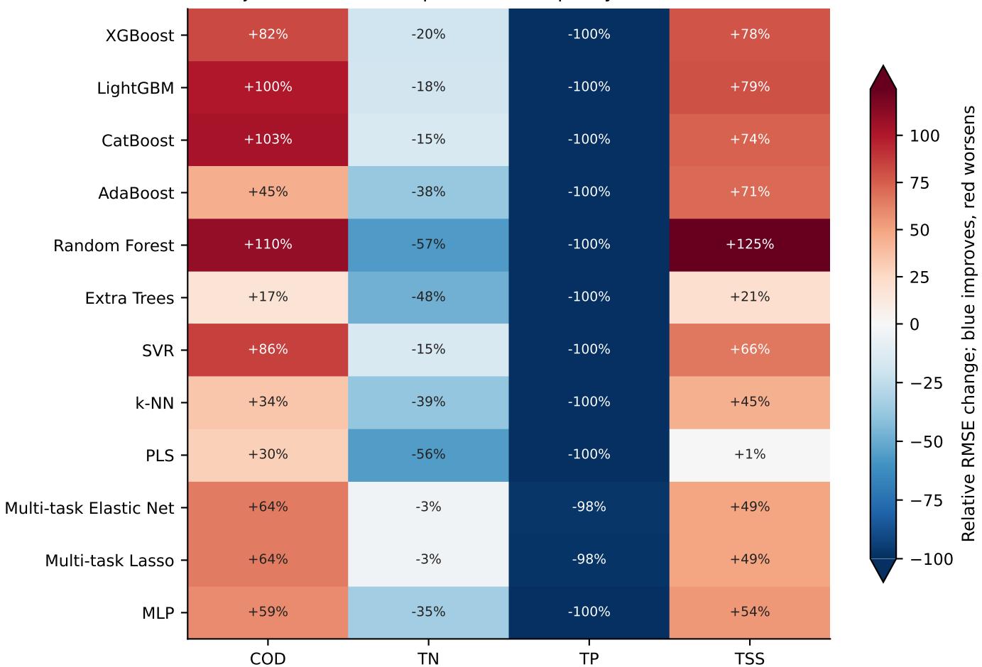
Projection effect on reported water-quality RMSE (N = 10,000)
