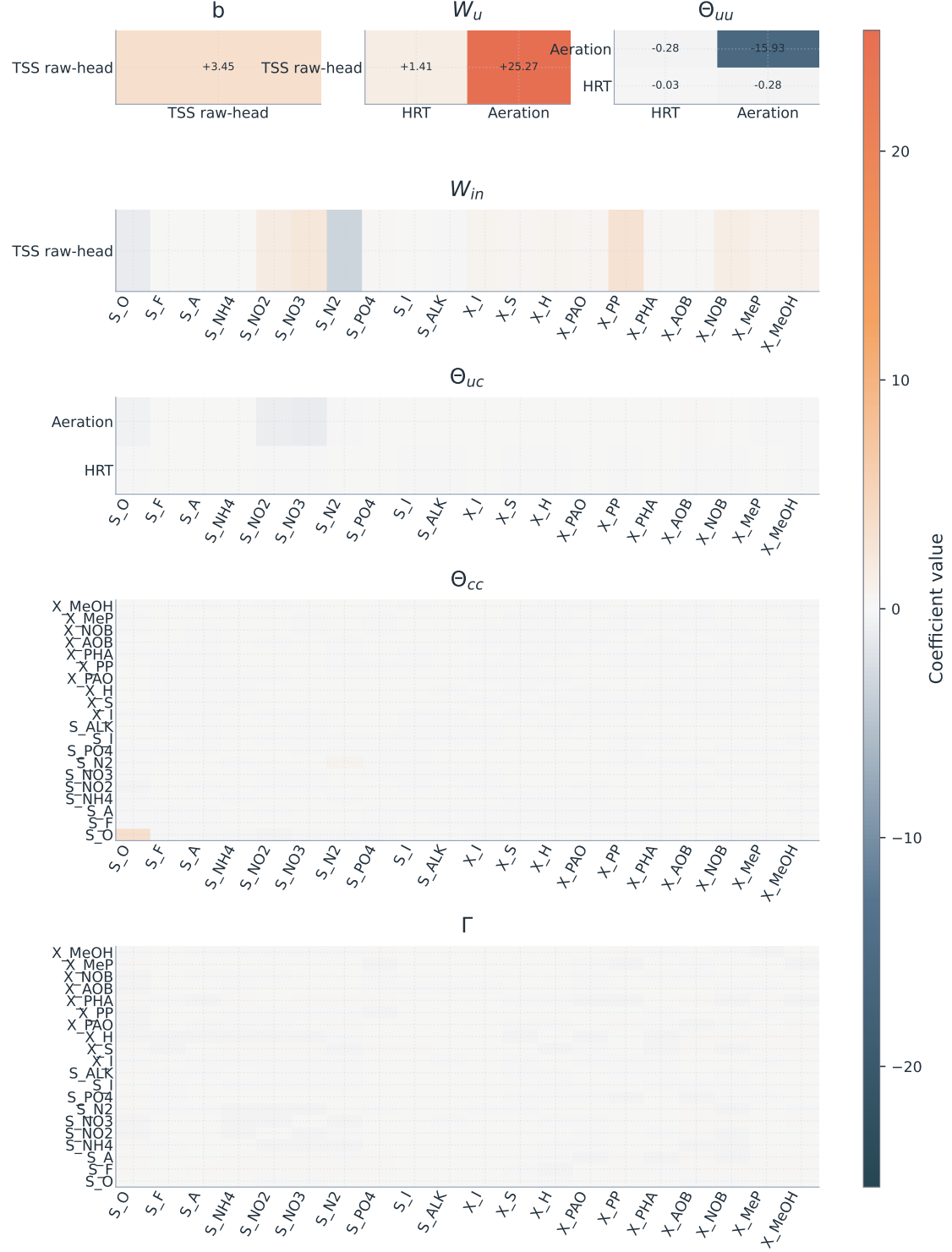
Figure S4: TSS raw-head ICSOR coefficient atlas showing the reported-target blocks of I_{comp}(I_F - \Gamma)^{-1}B together with the shared component-space coupling matrix \Gamma . The symmetric \Theta_{uu} and \Theta_{cc} panels display mirrored off-diagonal cells.
