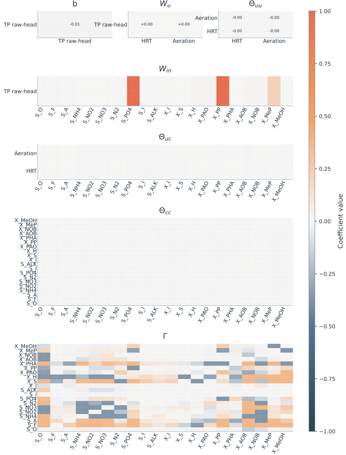
Figure S3: TP raw-head ICSOR coefficient atlas showing the reported-target blocks of I_{comp}(I_F - \Gamma)^{-1}B together with the shared component-space coupling matrix \Gamma . The symmetric \Theta_{uu} and \Theta_{cc} panels display mirrored off-diagonal cells.
