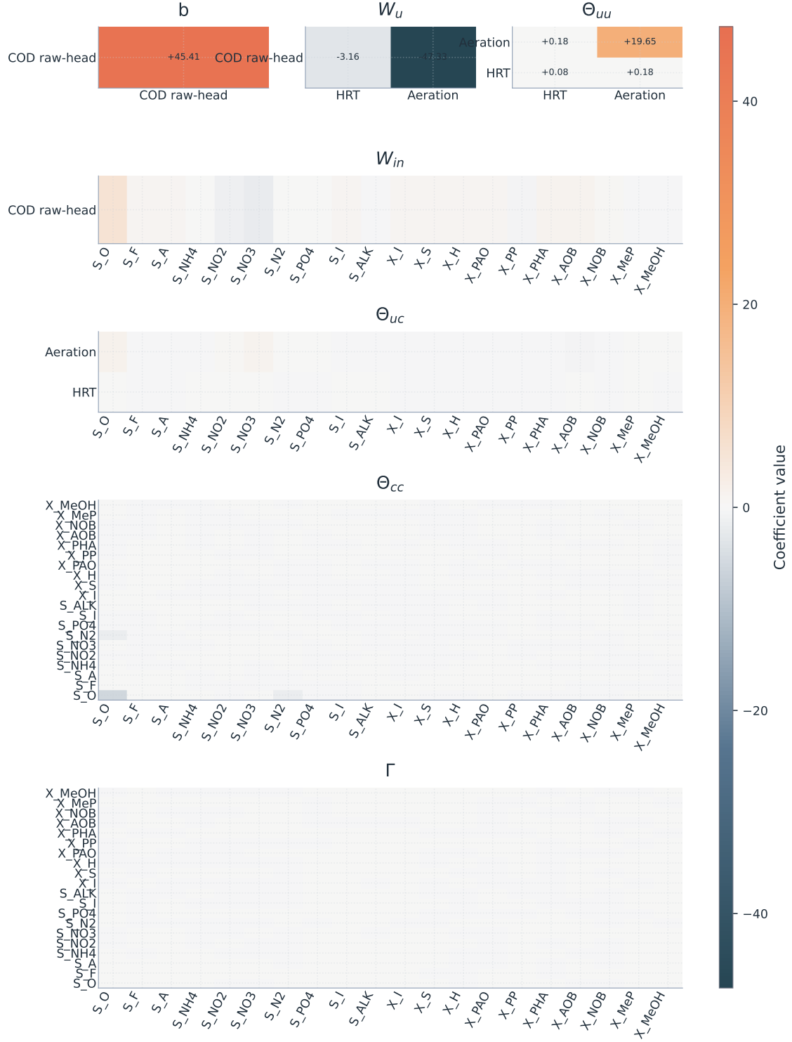
Figure S1: COD raw-head ICSOR coefficient atlas showing the reported-target blocks of I_{comp}(I_F - \Gamma)^{-1}B together with the shared component-space coupling matrix \Gamma . The symmetric \Theta_{uu} and \Theta_{cc} panels display mirrored off-diagonal cells.
