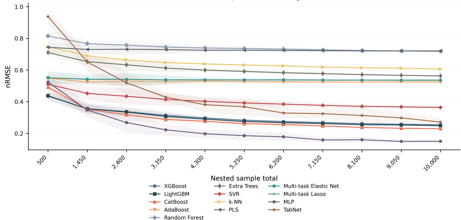
In-distribution raw-prediction learning curves
