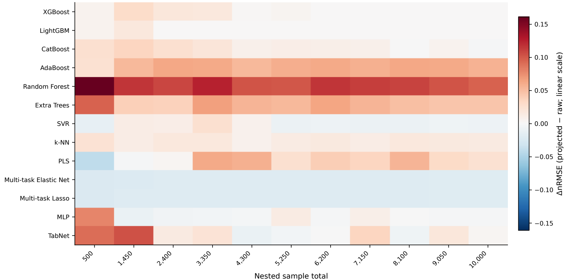
In-distribution effect of projection across sample size
