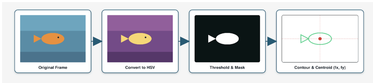
Figure 3. HSV Fish Tracking Pipeline.
