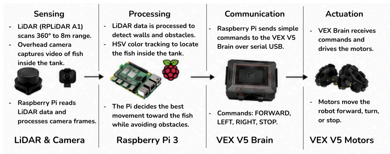
Figure 4. Fish Drive 2.0 System Architecture.
