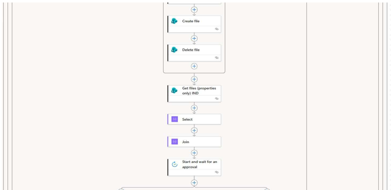
Figure 2: File copy (Create File), cleanup (Delete File), IND folder scan, Select/Join transformation, and Approval trigger
