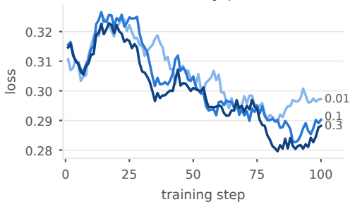
graph loss \mathcal{L}_{\text{graph}} (JSD)
