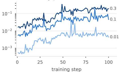
\|g_{\text{graph}}\| / \|g_{\text{KD}}\| (log)
