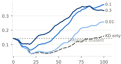
\|g_{\text{graph}}\| / \|g_{\text{KD}}\| (log)
