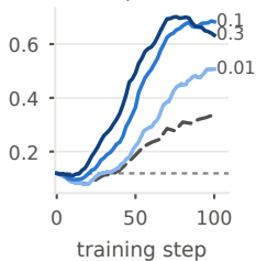
21_mult multiplication
