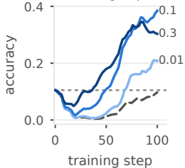
222_add three two-digit operands
