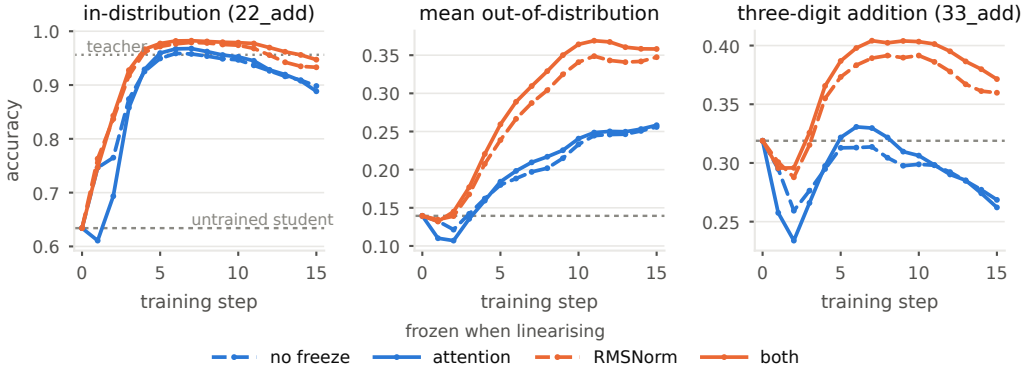
Figure 2: Accuracy against training step for the four linearisations. Hue carries the RMSNorm freeze and line style the attention freeze, so the 2 \times 2 design is visible as two pairs: the RMSNorm-frozen runs separate from the other two within a few steps and stay separated. The dashed rule marks the untrained student on every panel and the dotted rule in the left panel marks the teacher. In-distribution accuracy peaks around step 6–7 and then declines in all four runs, while out-of-distribution accuracy is still climbing at step 15 for the two runs without the RMSNorm freeze; the right panel shows those same two runs ending below the untrained student on three-digit addition, which the two RMSNorm-frozen runs do not.
