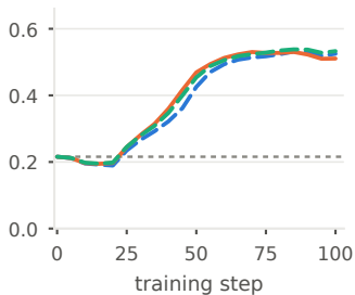
mean out-of-distribution
