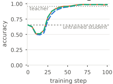
in-distribution (22_add)
