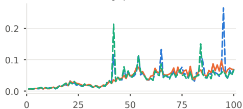
fraction of update signs set by the graph term
