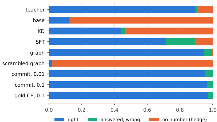
21_mult, BOS at eval
