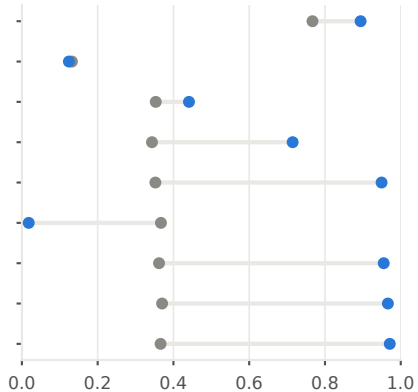
accuracy without BOS (grey) and with BOS (blue)
