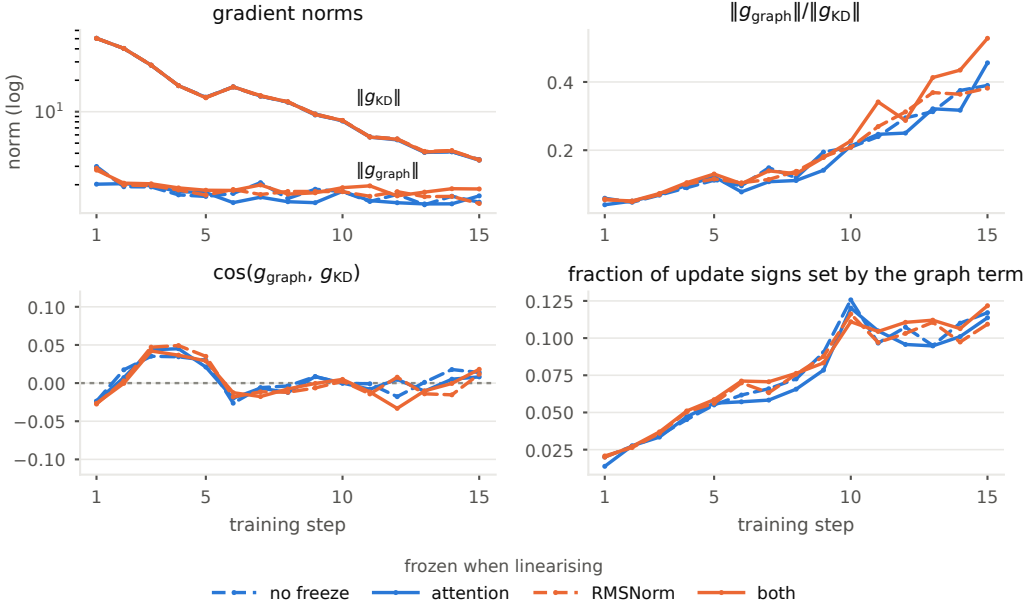
Figure 4: Per-step gradient metrics for the four linearisations, encoded as in Figure 3. All four variants are drawn on every panel and lie almost exactly on top of one another — that overlap is the point, not a plotting artefact. The KD gradient collapses by a factor of 14.6 while the graph gradient stays flat, so their ratio climbs tenfold and the share of update signs the graph term decides rises from 2% to 12%, none of it by design. The cosine oscillates about zero throughout and never drifts. Yet these four runs differ by a third in out-of-distribution accuracy, so what separates them is not visible in any of these aggregates.
