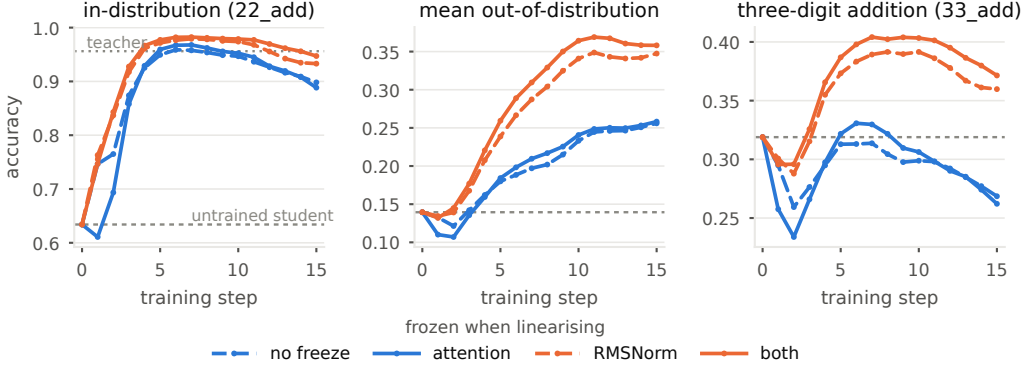
Figure 3: Accuracy against training step for the four linearisations. Hue carries the RMSNorm freeze and line style the attention freeze, so the 2×2 design is visible as two pairs: the RMSNorm-frozen runs separate from the other two within a few steps and stay separated. The dashed rule marks the untrained student on every panel and the dotted rule in the left panel marks the teacher. In-distribution accuracy peaks around step 6–7 and then declines in all four runs, while out-of-distribution accuracy is still climbing at step 15 for the two runs without the RMSNorm freeze; the right panel shows those same two runs ending below the untrained student on three-digit addition, which the two RMSNorm-frozen runs do not.
