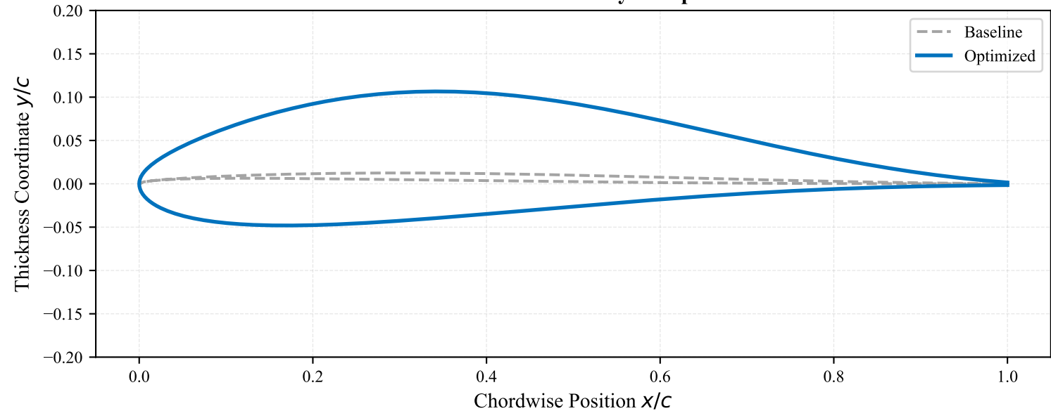
Airfoil Profile Geometry Comparison
