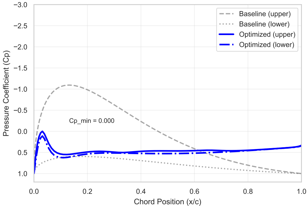
Surface Pressure Distribution
