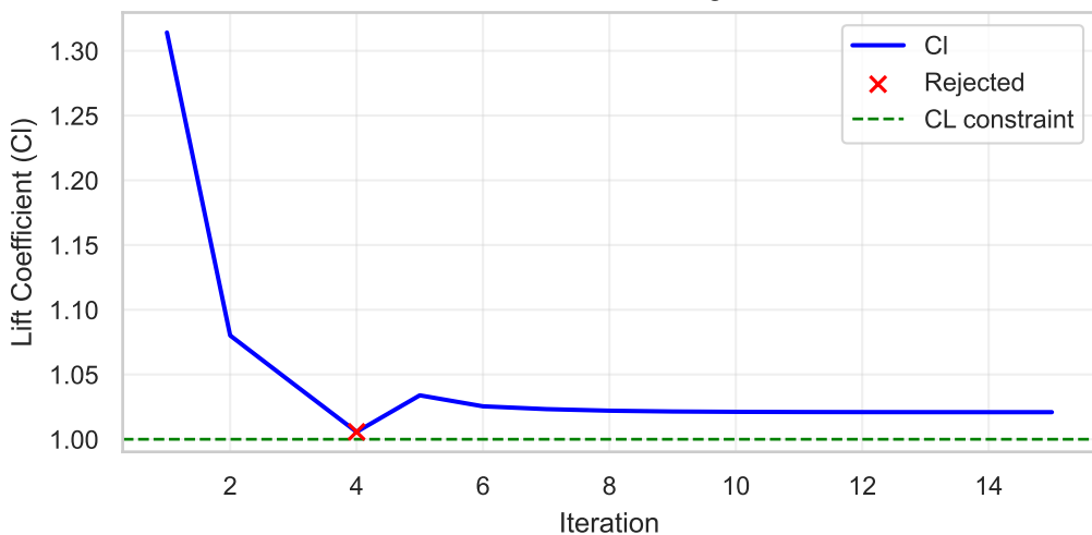
Lift Coefficient Convergence
