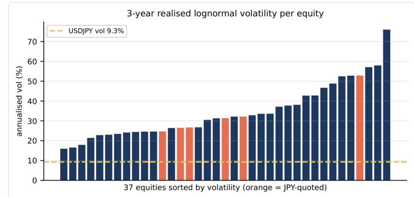
3-year realised lognormal volatility per equity (orange = JPY-quoted).
