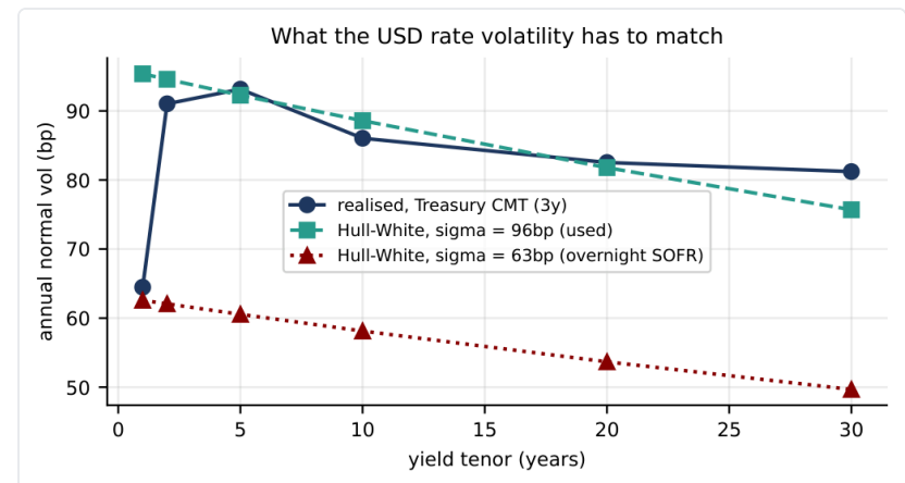
Realised Treasury yield vol by tenor vs. the Hull-White implied shape for both sigma choices.
