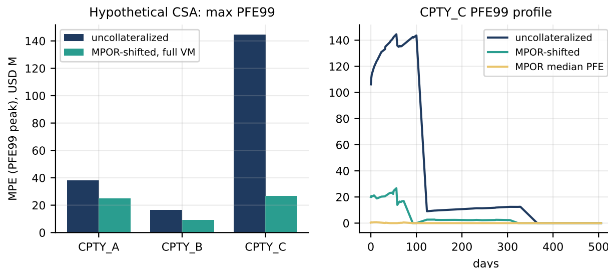
Figure 28: If a full-VM CSA existed, peak PFE99 would fall sharply, most of all for CPTY_C whose exposure is a large, already-visible MTM that margin would cover.
