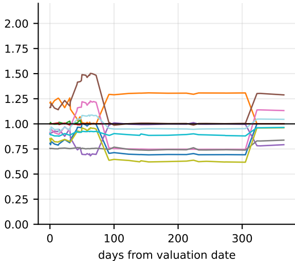
Close-out PFE99, portfolio: stressed / base
