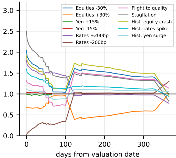
Level PFE99, portfolio: stressed / base
