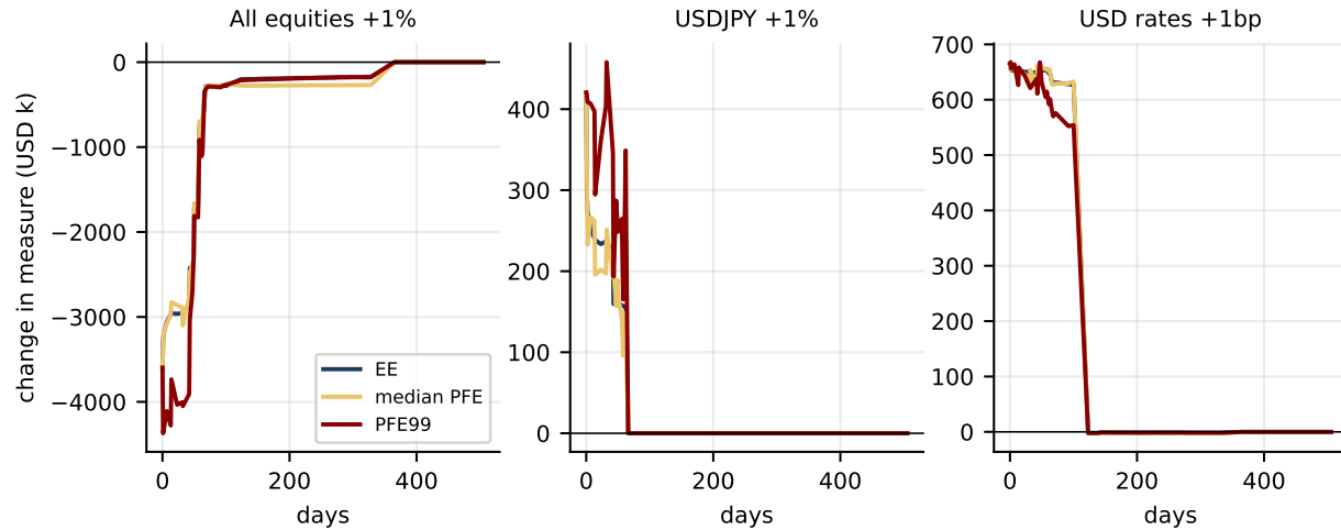
Figure 32: Change in portfolio EE, median PFE and PFE99 through time for +1% on all equities, +1% on USDJPY and +1bp on USD rates.
