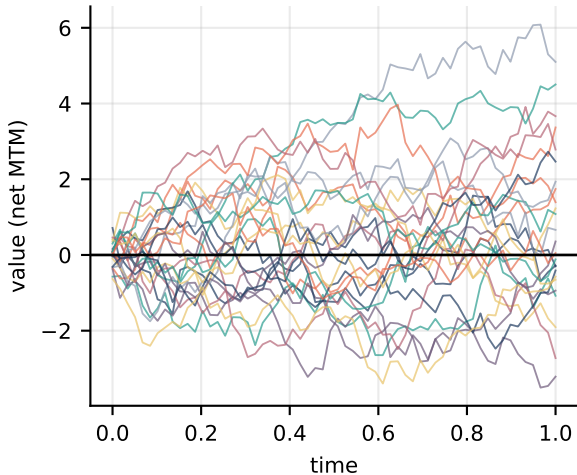
Simulated portfolio value V(t) on 25 scenarios
