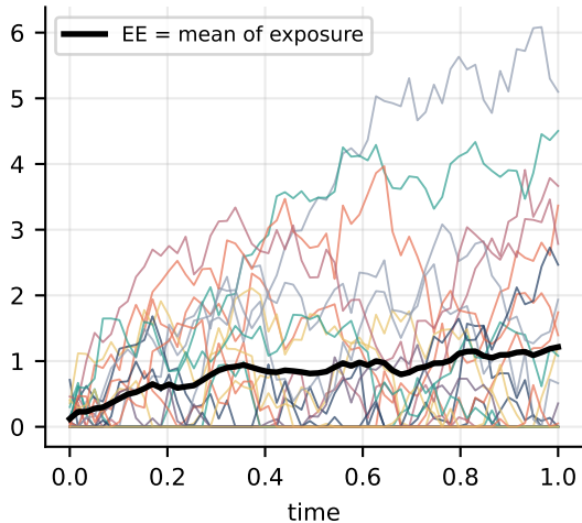
Exposure = \max(V, 0) : only gains are at risk
