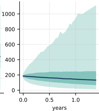
equity US816850 (vol 76%)
