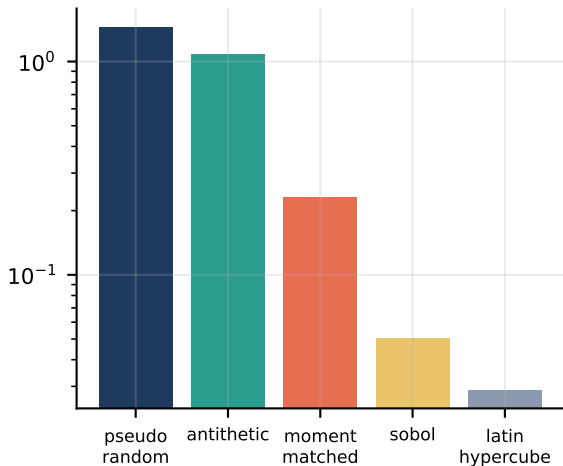
European call test: RMSE vs Black-Scholes (log)
