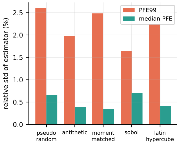
Real engine: estimator noise at equal N
