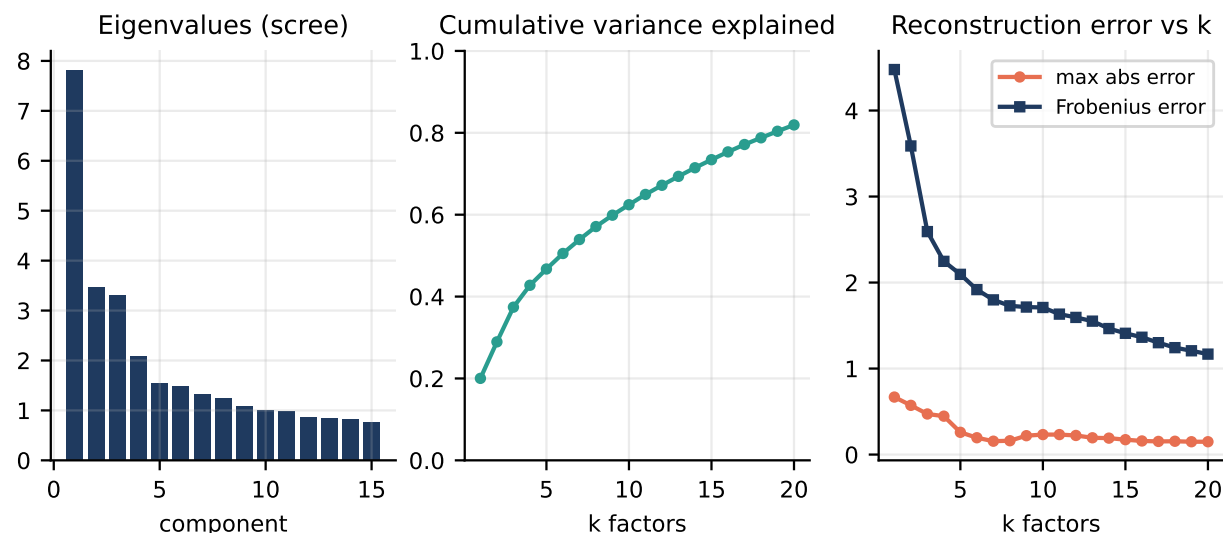
Figure 6: Left: the first eigenvalue (7.8 of a total 39) is one dominant market factor. Middle: 5 factors explain 47% of variance and 10 explain 62%. Right: reconstruction error falls as k grows (exactly zero at full rank).
