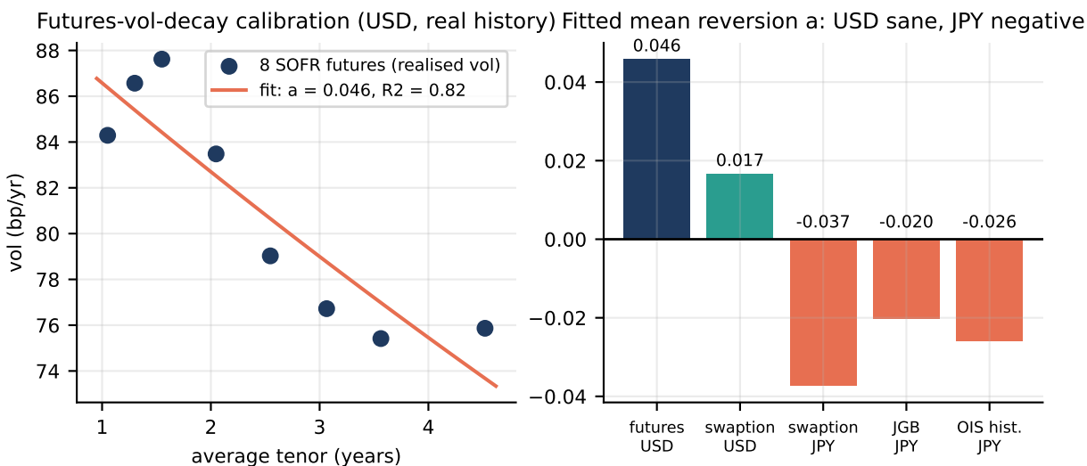
Figure 12: Left: USD SOFR-futures fit. Right: fitted a for each route. USD routes give sensible positive values; all three JPY routes give a NEGATIVE a.
