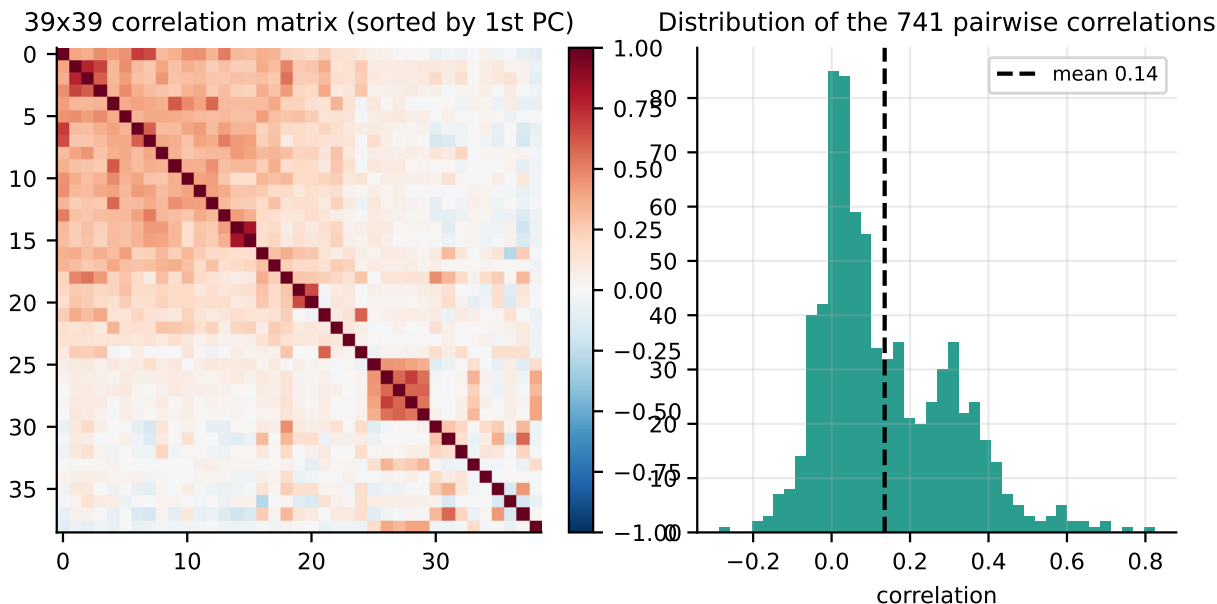
Figure 5: Left: the 39x39 correlation matrix reordered so similar names sit together; a broad positive ‘market’ block is visible. Right: the 741 pairwise correlations centre on 0.14.
