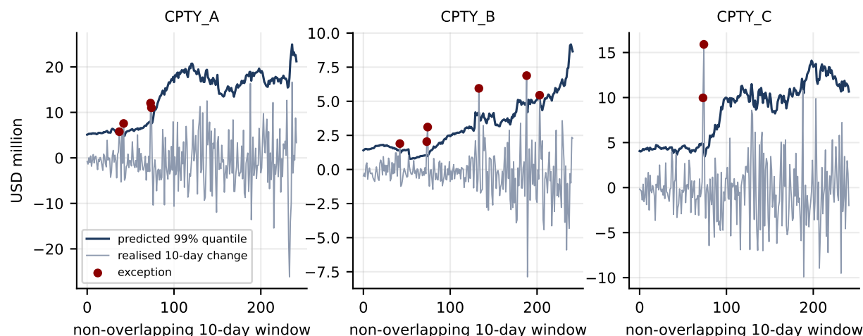
Figure 25: Predicted 99% quantile of the 10-day change in each netting set's equity positions against the realised change, over the whole backtest; exceptions in red.
