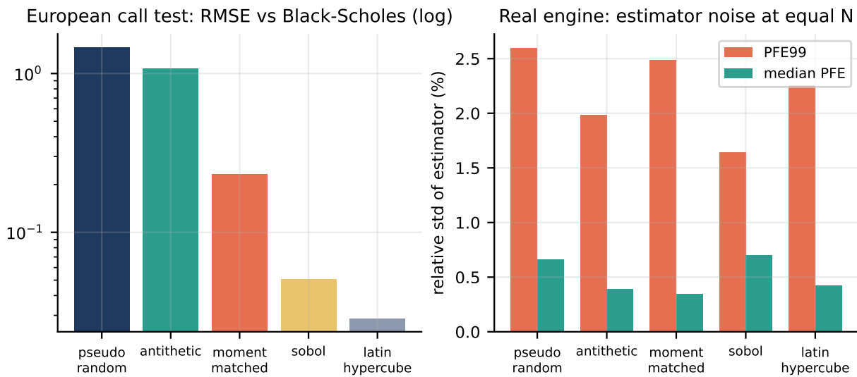
Figure 10: Left: on a European call with a known Black-Scholes value, Latin Hypercube has about 51x lower error than pseudo-random. Right: on the real 663-dimensional engine (300 scenarios, 8 repeats) the methods are much closer, and no method is best for both PFE99 and the median PFE.
