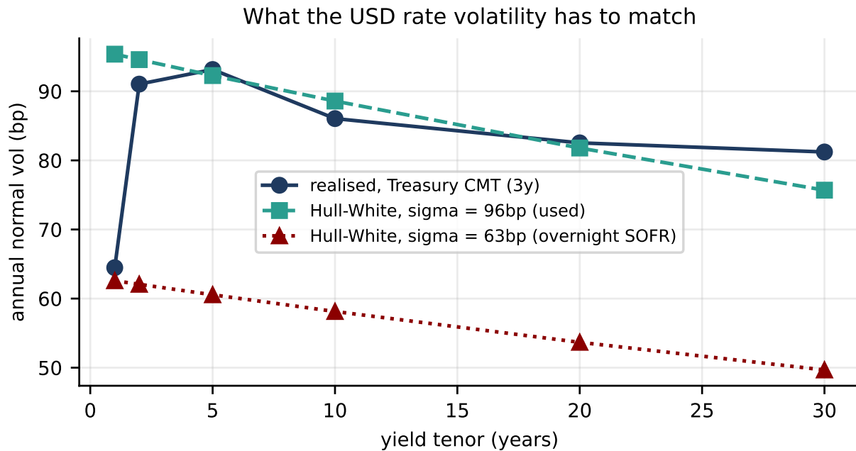
Figure 4: Realised yield volatility by tenor against the Hull-White implied shape for the two choices of sigma. The overnight-SOFR calibration lies well below the long-end moves; the fit tracks them.
