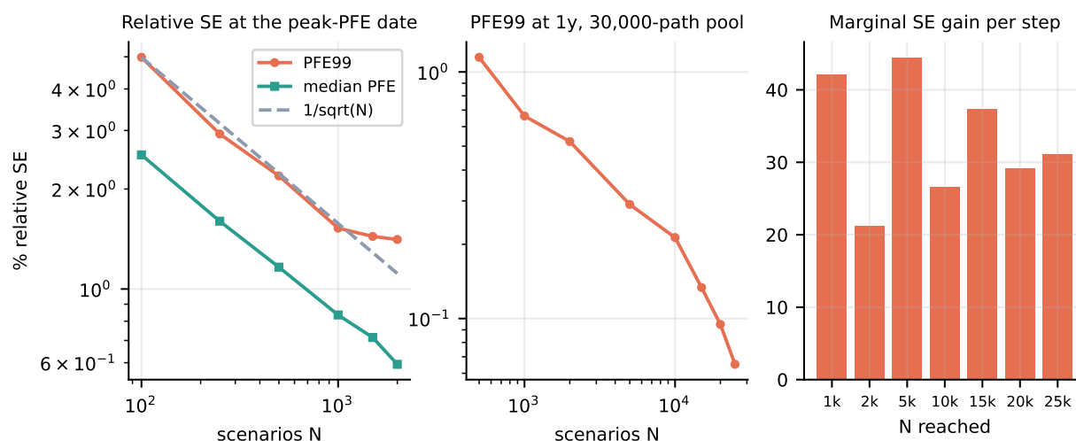
Figure 11: Left: relative standard error of PFE99 and median PFE at the peak-PFE date (2026-10-09); the error follows the 1/\sqrt{N} law. Middle and right: PFE99 tail study at one year; error is larger for the same N , and the marginal gain per additional batch peaks at N = 5,000 and then declines.
