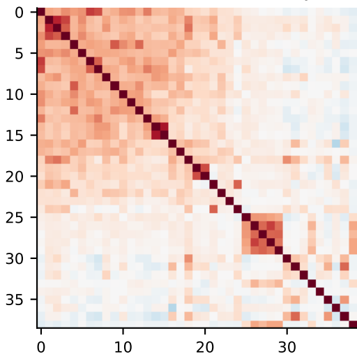
39x39 correlation matrix (sorted by 1st PC)
