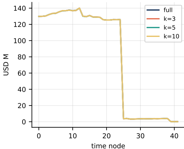
Portfolio EE: full-rank vs PCA factor model
