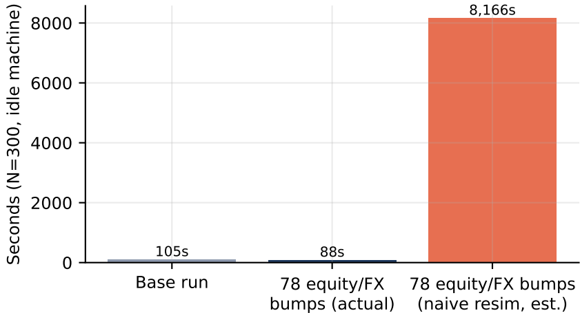
Cost: bump-and-reprice vs naive resimulation
