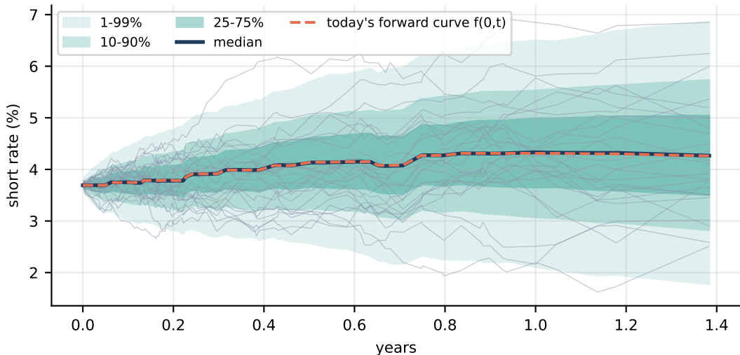
Simulated USD short rate: Hull-White fan (3,000 scenarios)
