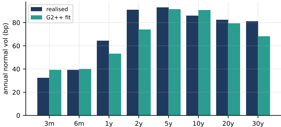
G2++ calibration: yield volatility by tenor
