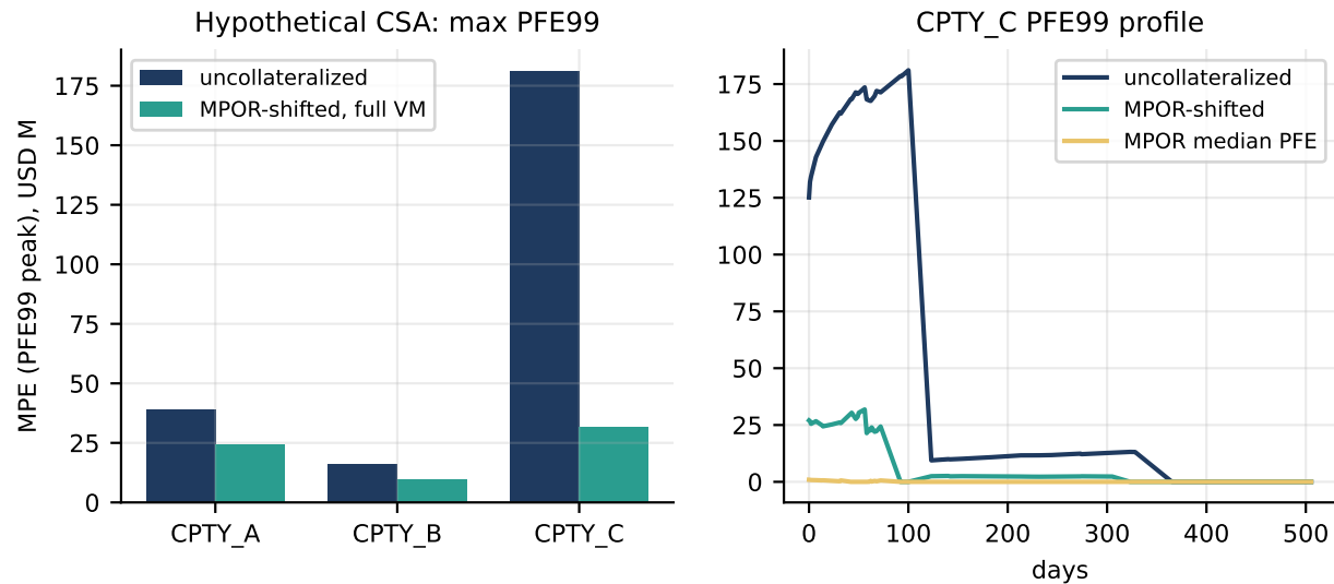
Figure 31: If a full-VM CSA existed, peak PFE99 would fall sharply, most of all for CPTY_C whose exposure is a large, already-visible MTM that margin would cover.
