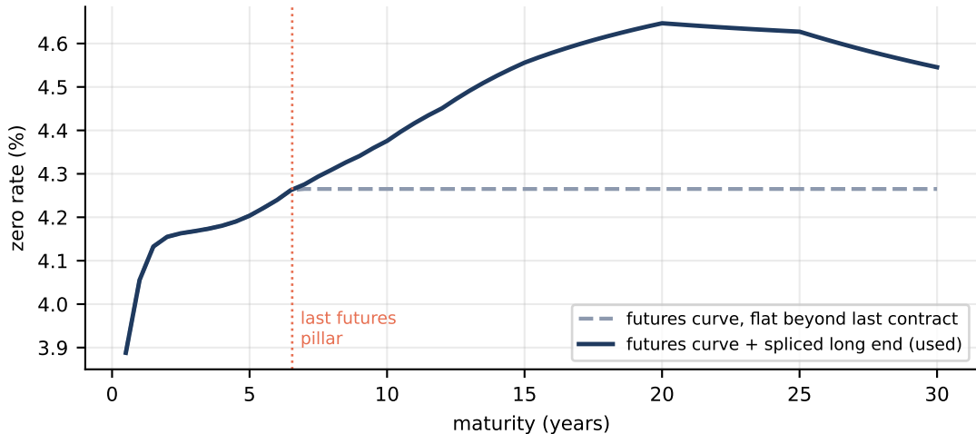
USD zero curve before and after the long-end splice
