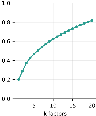
Cumulative variance explained
