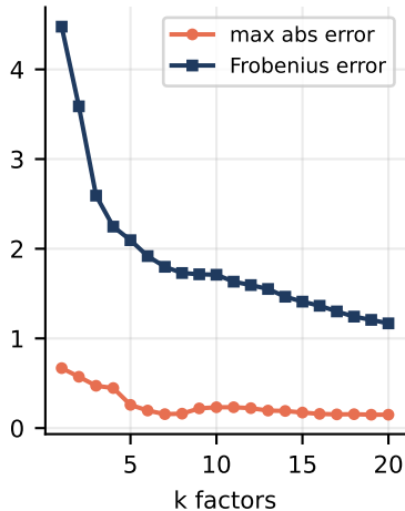
Reconstruction error vs k
